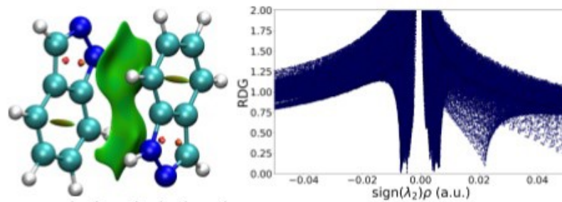
Indazole-Indazole
