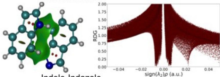
Indole-Indazole
