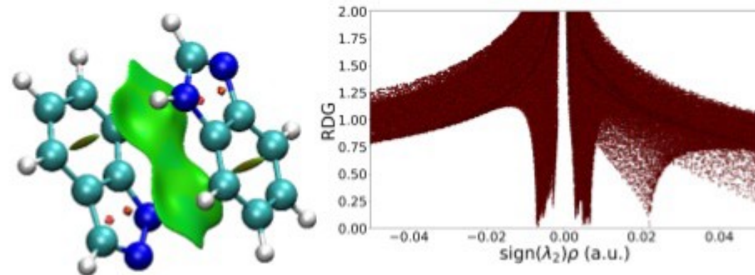
Benzimidazole-Indazole
