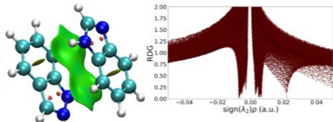
Benzimidazole-Indole
