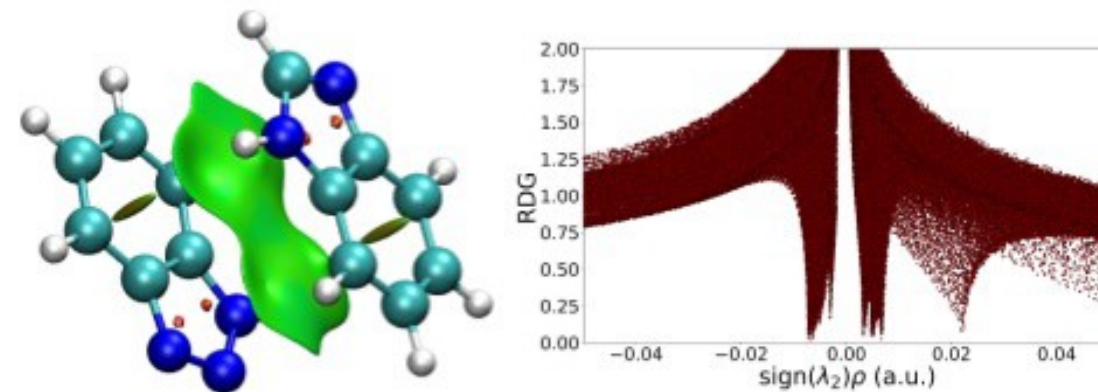
Benzimidazole-Benzotriazole
