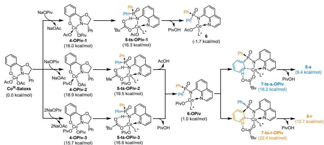
Fig. S2 Relative Gibbs free energy of pivolate-ligated cobalt species promoted C-H functionalization
