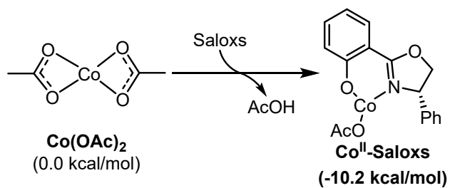
Fig. S1 Transformation of \text{Co}(\text{OAc})_2 to \text{Co}^{\text{II}} -Saloxs
