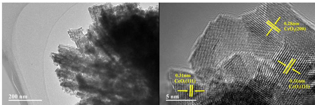
Fig. S2. Typical TEM and HRTEM image of catalyst M 3 C 7 .
