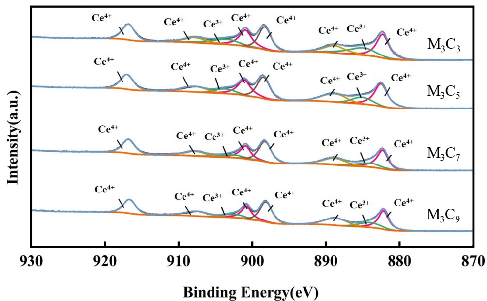
Fig. S4. Ce 3d XPS spectra of M_3C_{3-9} .
