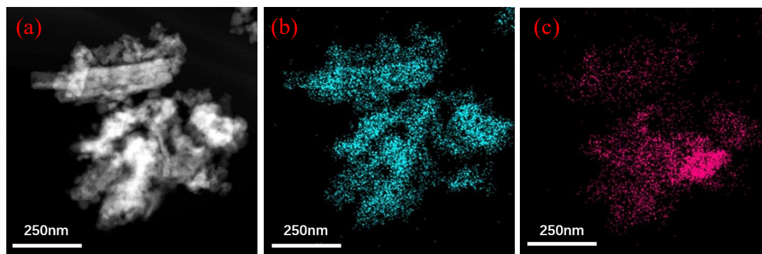
Fig. S3. (a) STEM image, (b) Ce mapping, and (c) Mn mapping of catalyst M 3 C 7 .
