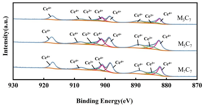
Fig. S5. Ce 3d XPS spectra of M_{3-7}C_7 .
