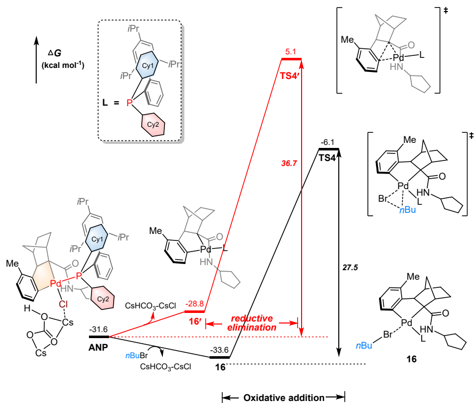
Fig. S3 Calculated Gibbs energy profiles for C(sp 3 )–Br oxidative addition vs. C–C norbornene reductive elimination.
