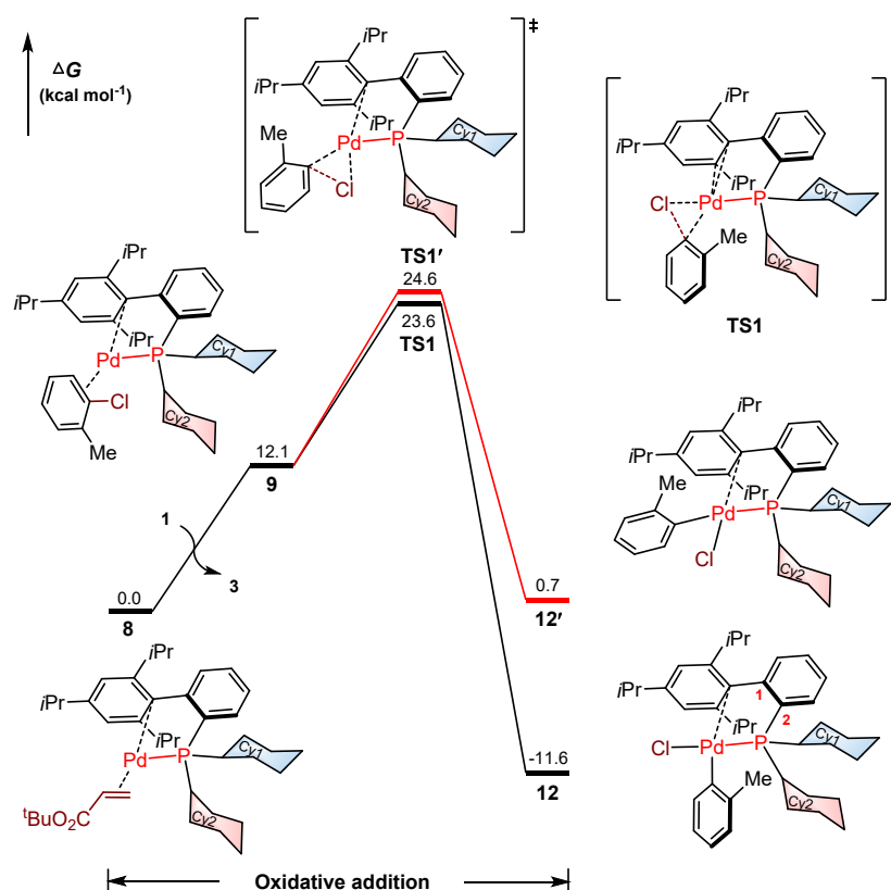
Fig. S1 Calculated Gibbs free energy profiles for oxidative addition of Ar–Cl to Pd 0 with the Cl atom and P atom in a cis orientation.
