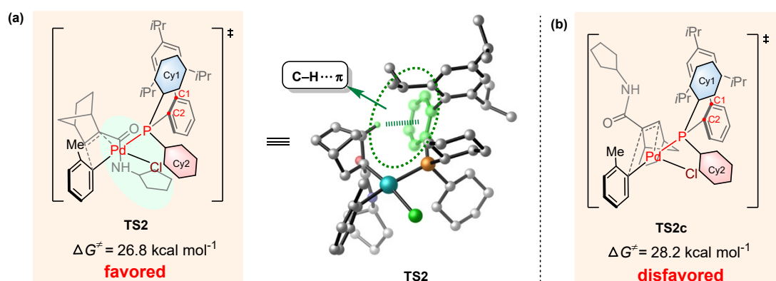
Fig. S2 (a) Analysis of C–H⋯π interaction in TS2, and (b) calculated Gibbs energy for 2,1-insertion of NBE.
