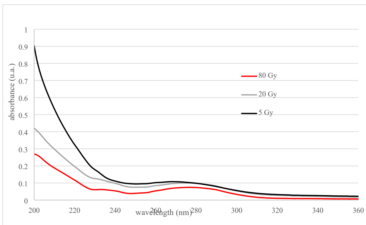
Supplementary material 3. Spectra of samples during degradation of irradiated solution with initial concentration 3 mg/L
