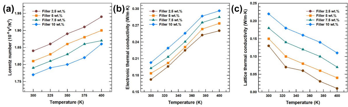
Fig. S4. Temperature-dependent (a) Lorentz number, (b-c) electronic and lattice thermal conductivity of each composite.
