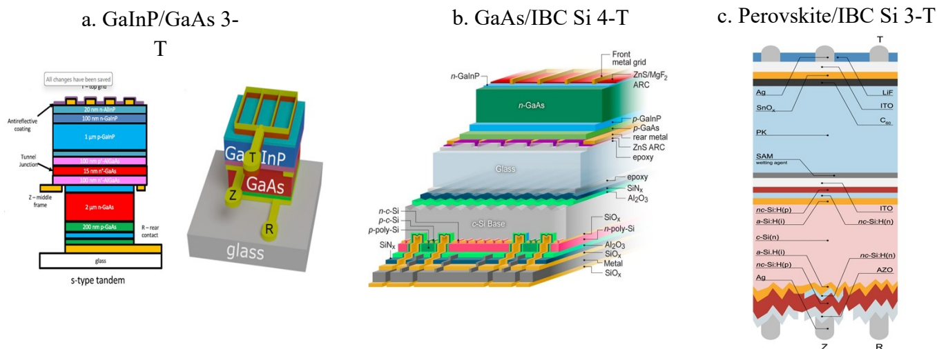
Fig. S1. Device schematics of the three multi-terminal cells in the paper: (a) GaInP/GaAs 3-T, Geisz et. al. [15] (b) GaAs/IBC Si 4-T, VanSant et. al. [10], and (c) perovskite/IBC Si 3-T, Kikelj et. al. [11].
