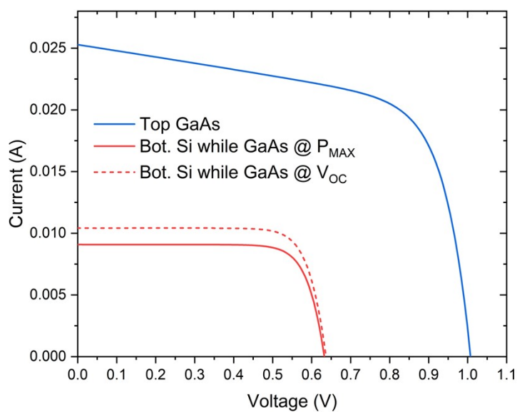
Fig. S2. Separate light I-V curves of the GaAs/Si 4-T tandem cell shown in Fig. 4.
