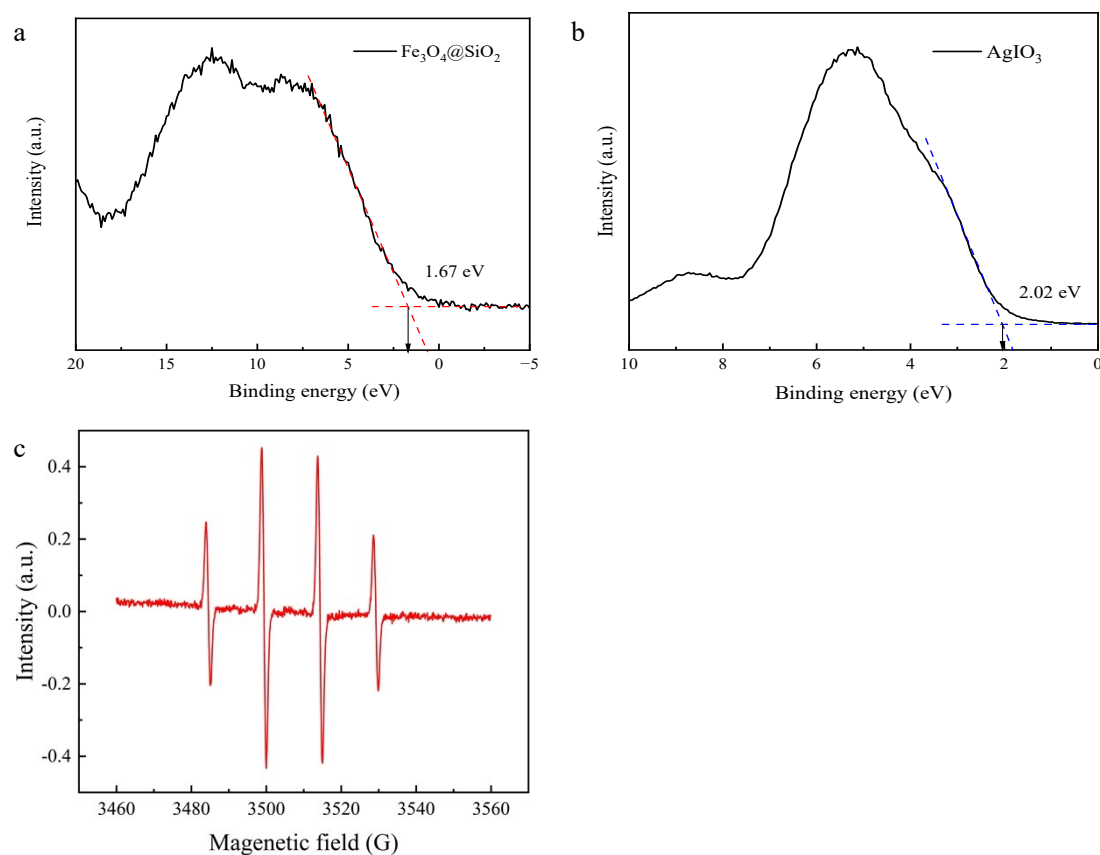
Fig. S1. Valence-band XPS spectra of (a) \text{Fe}_3\text{O}_4@\text{SiO}_2 , (b) \text{AgIO}_3 ; DMPO spin-trapping EPR spectra recorded with AFS-15 in aqueous dispersion (for \text{DMPO} \cdot \text{OH} ) under visible irradiation.
