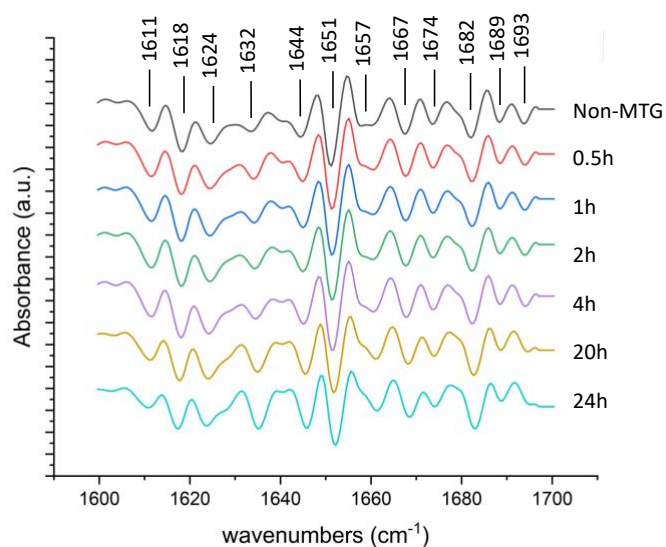
Fig. S1 FTIR spectra (650-4000 cm -1 ) of BSFL protein dispersions subjected to MTG treatment for different durations
