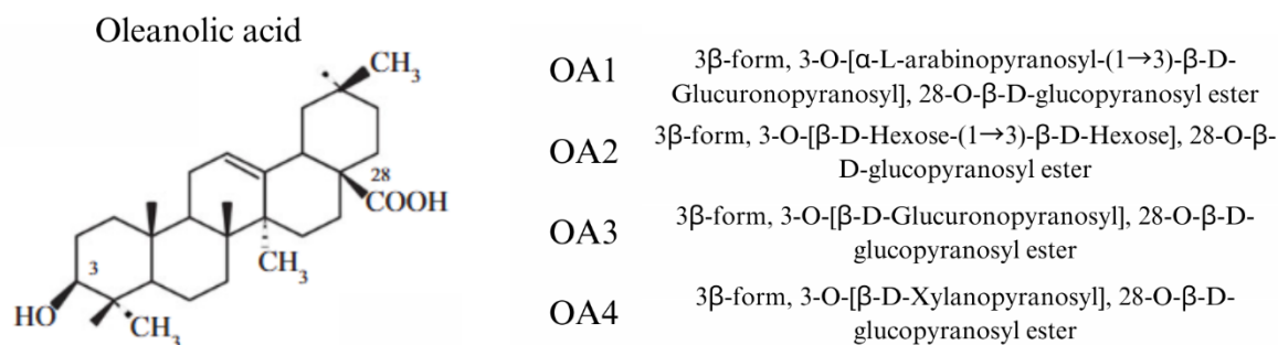
Supplementary material 4. Saponins chemical structures determined after HPLC-MS-TOF analysis of C. berlandieri seeds.
