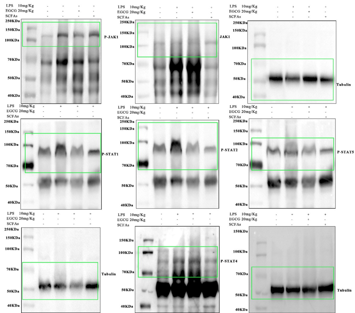
Fig S7.A Full membrane diagramGroup 2
