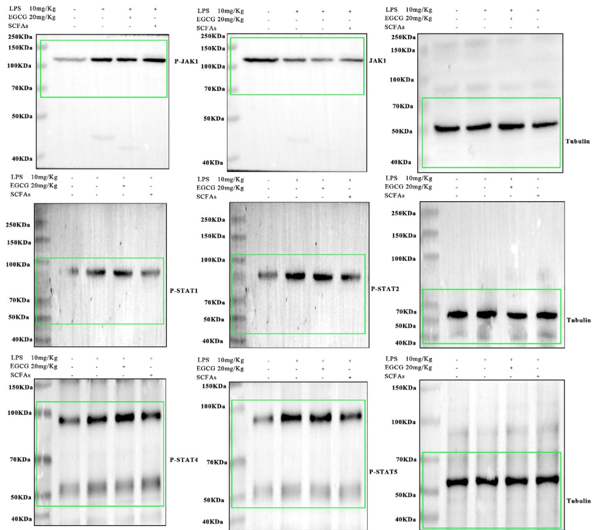
Fig S7.A Full membrane diagramGroup 1
