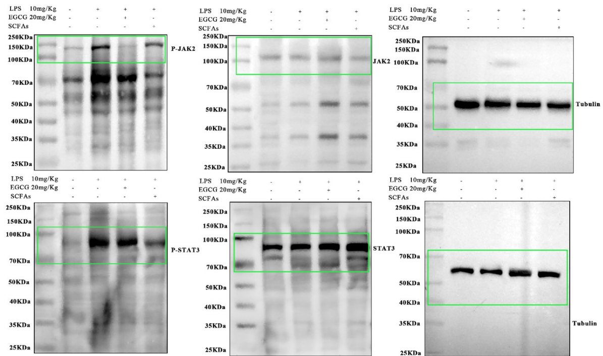
Fig 12.C Full membrane diagramGroup 2
