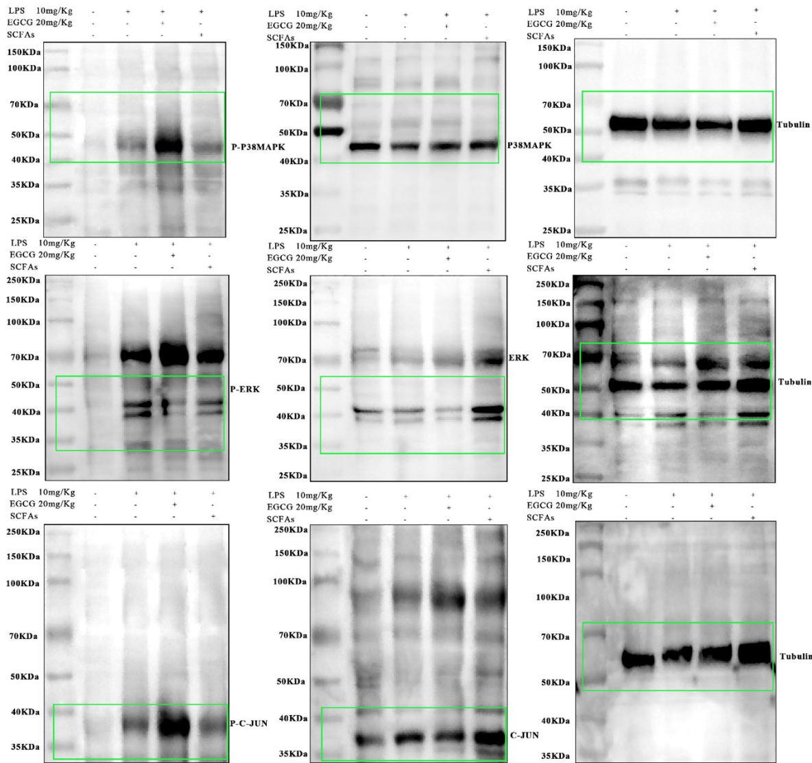
Fig S7.G Full membrane diagramGroup 2
