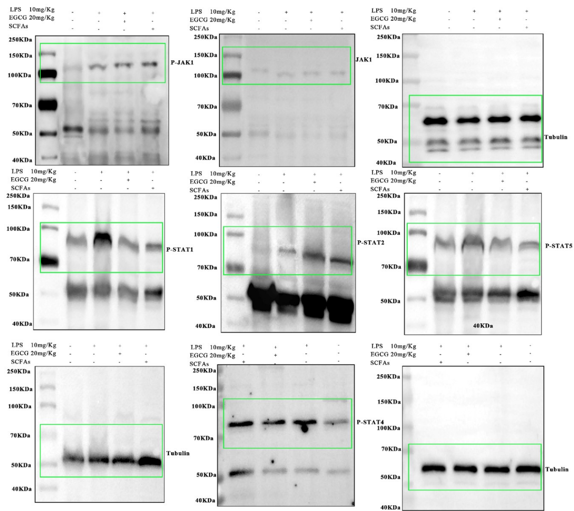
Fig S7.A Full membrane diagramGroup 3
