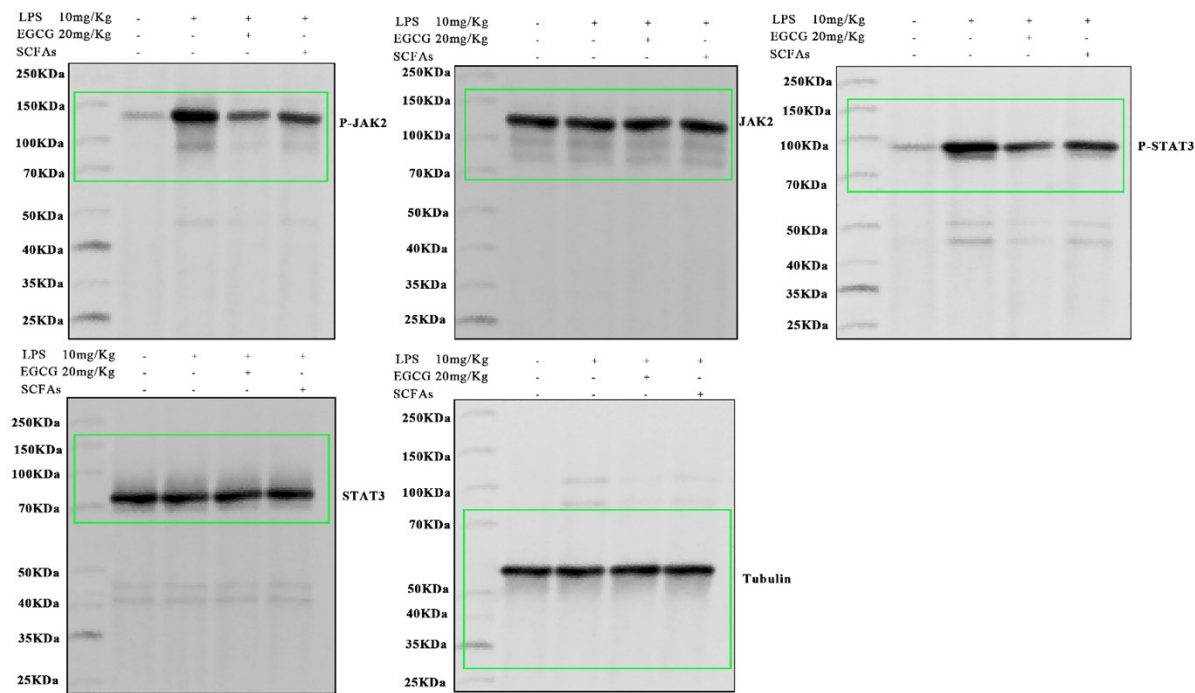
Fig 12.C Full membrane diagramGroup 2
