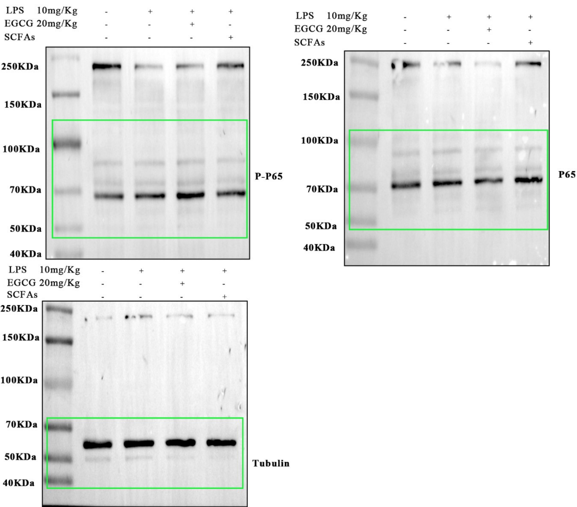
Fig S8.E Full membrane diagramGroup 1
