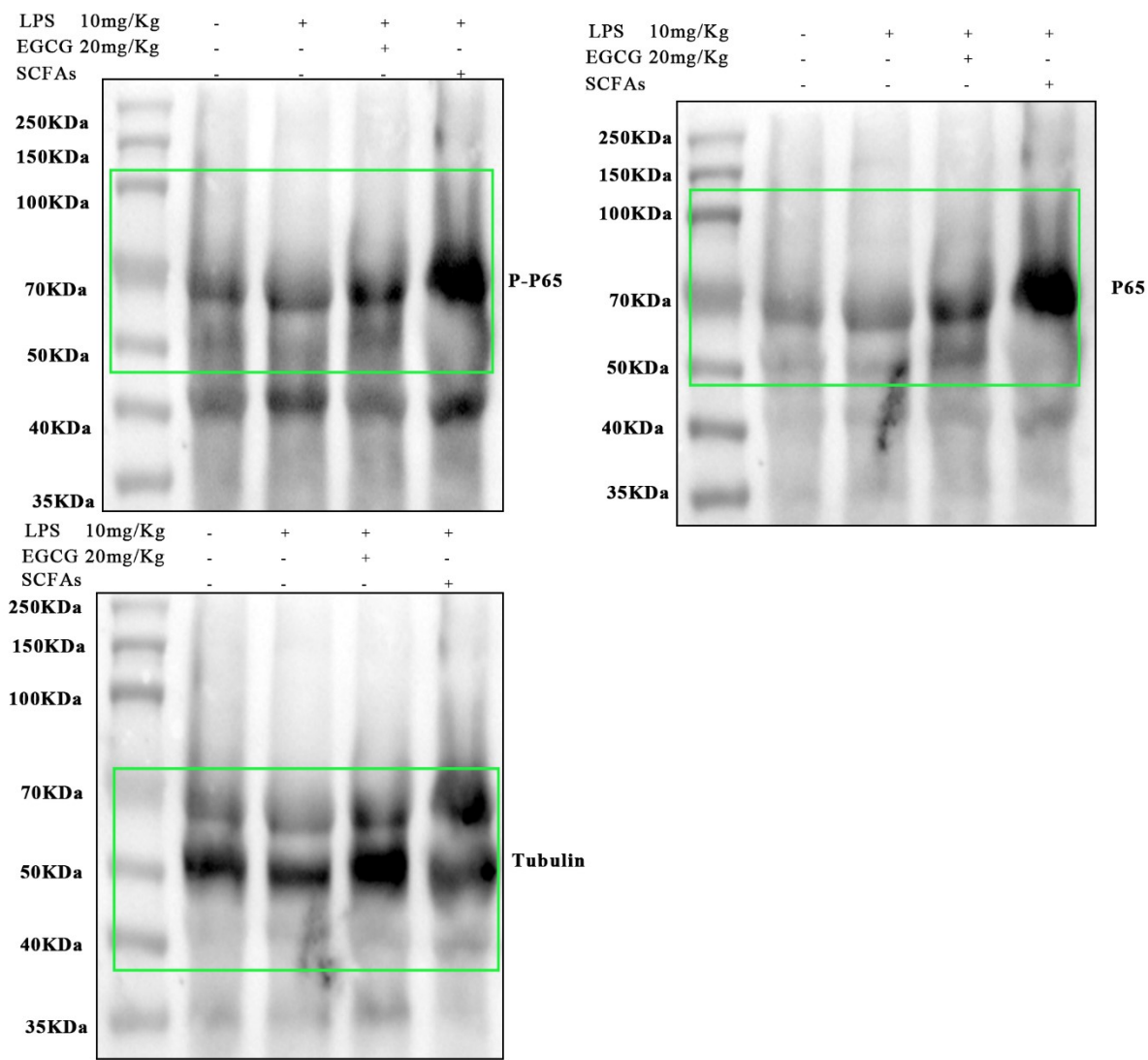
Fig S8.E Full membrane diagramGroup 3
