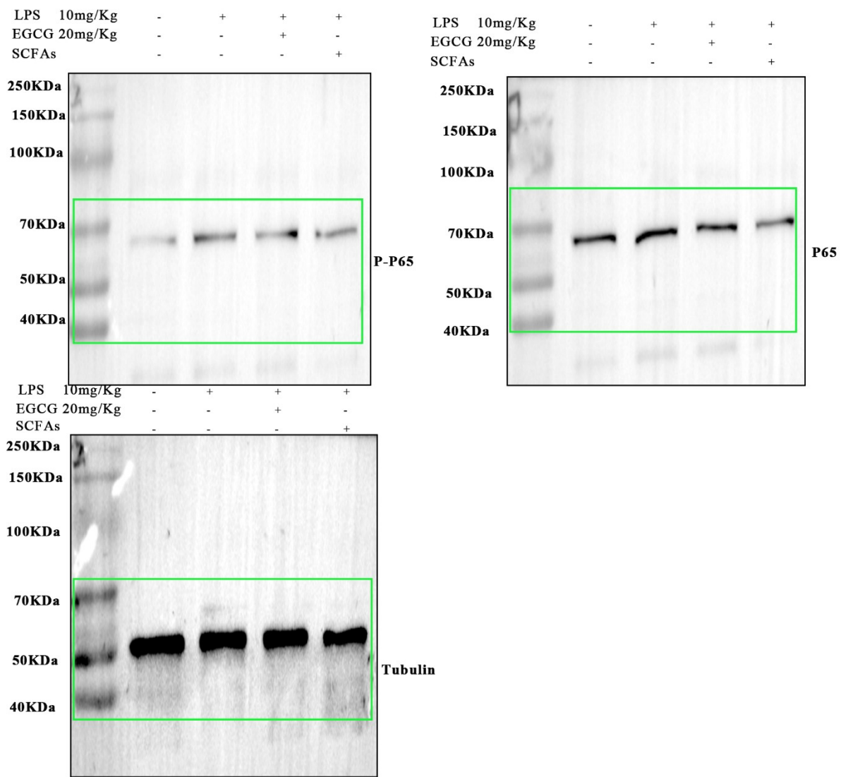
Fig S8.E Full membrane diagramGroup 2
