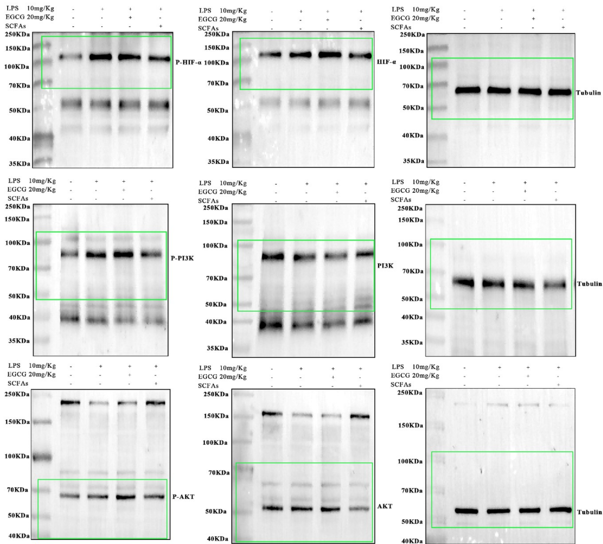
Fig S8.A Full membrane diagramGroup 1
