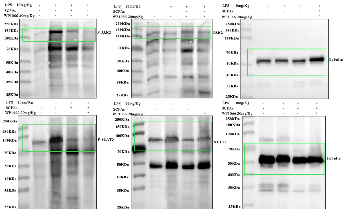
Fig 13.B Full membrane diagramGroup 2
