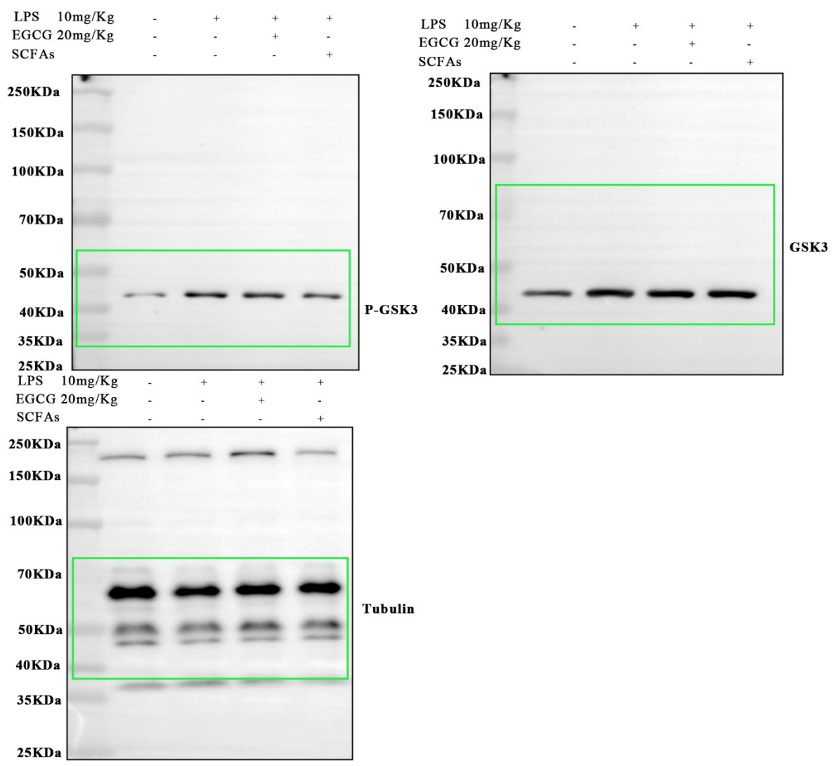
Fig S8.G Full membrane diagramGroup 1
