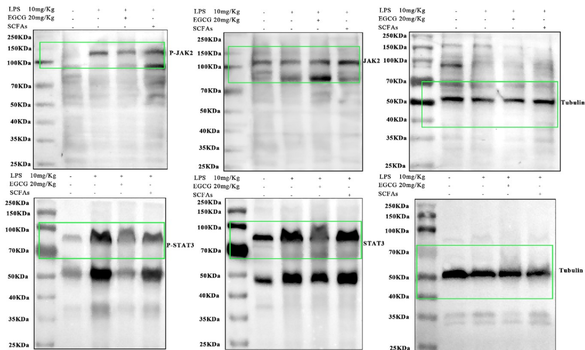
Fig 12.C Full membrane diagramGroup 3
