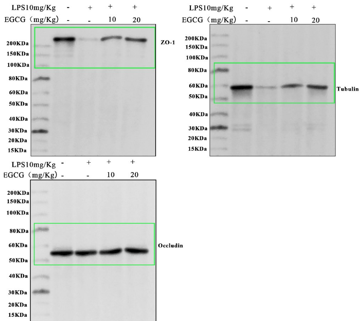
Fig 4.E Full membrane diagramGroup 3
