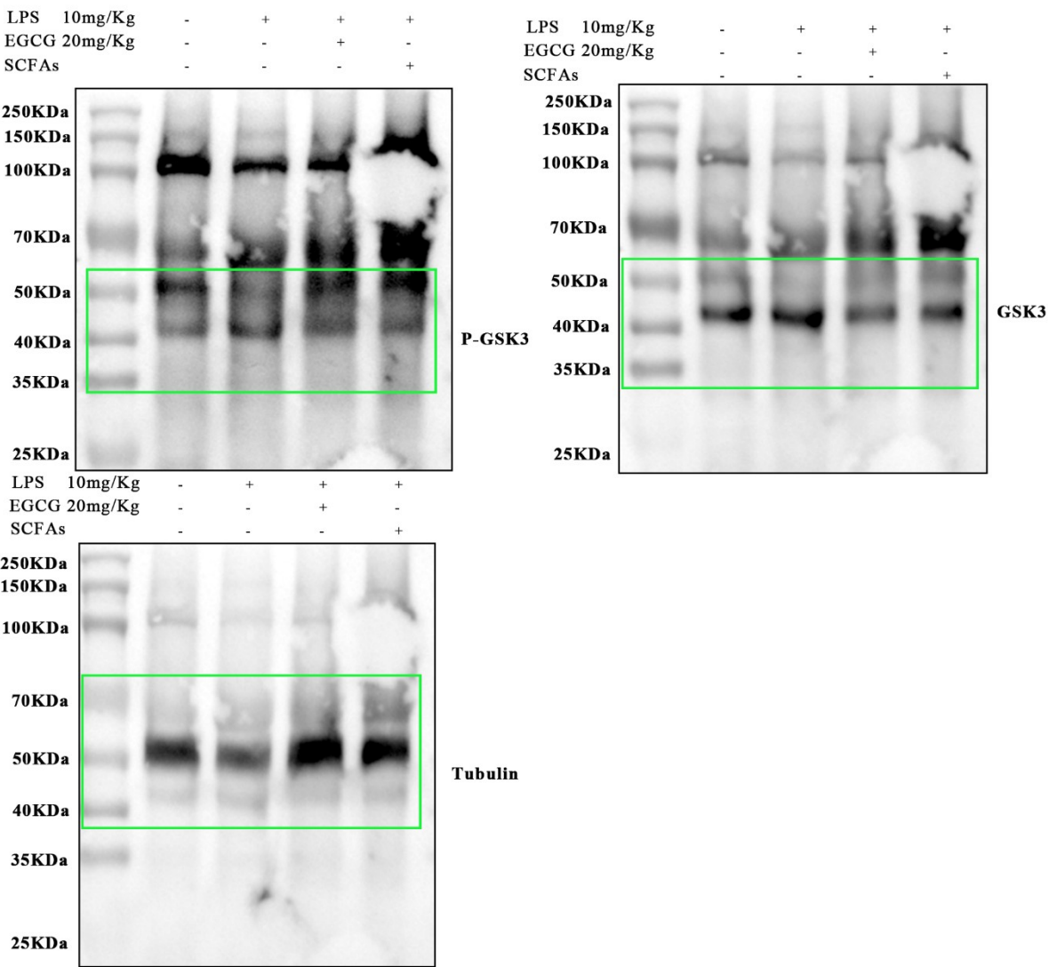
Fig S8.G Full membrane diagramGroup 2
