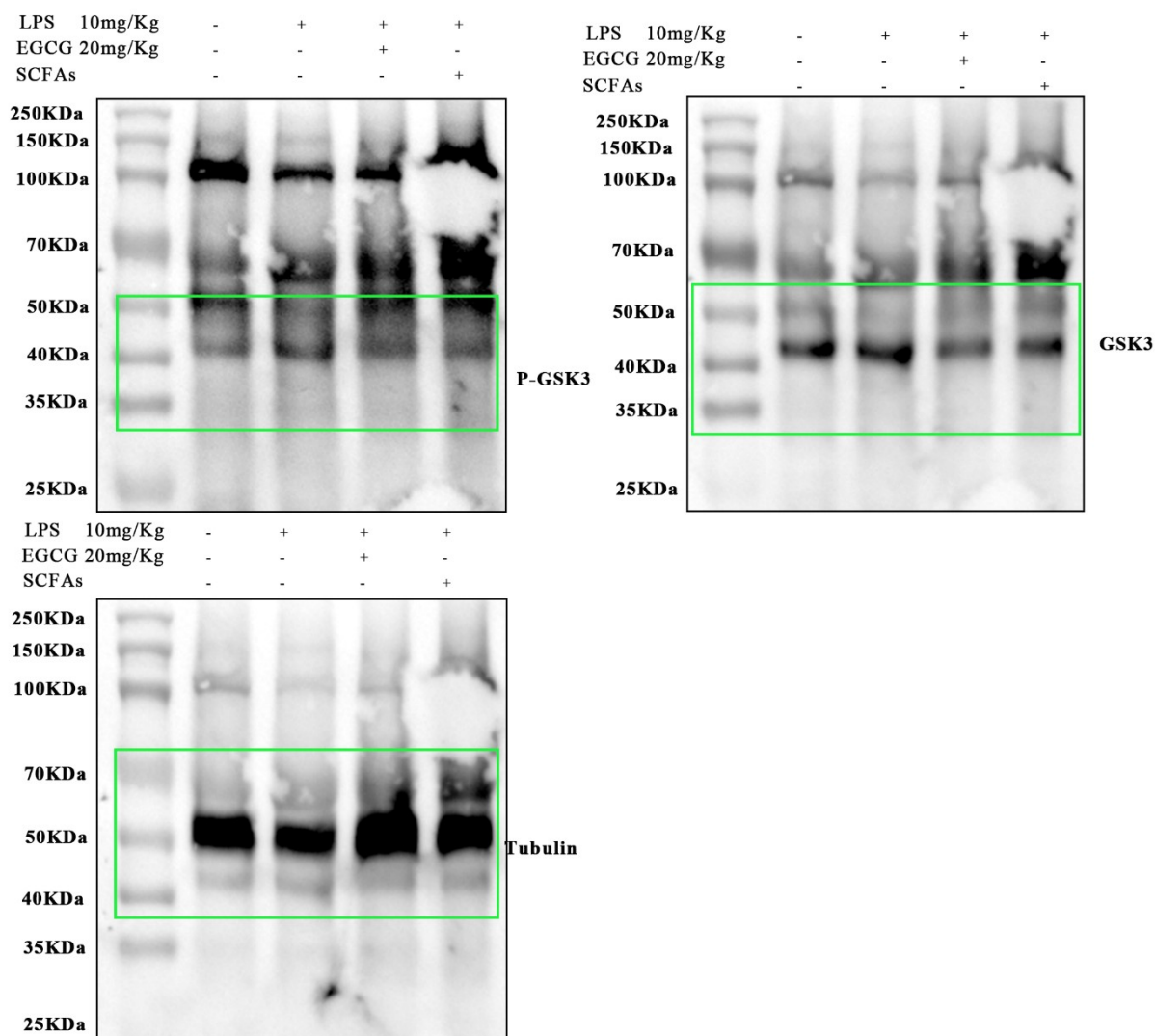
Fig S8.G Full membrane diagramGroup 3
