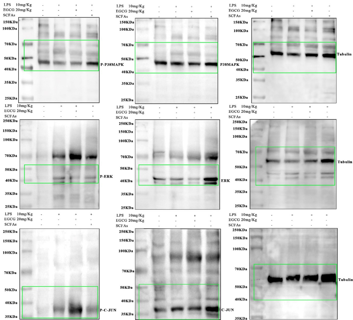
Fig S7.G Full membrane diagramGroup 3
