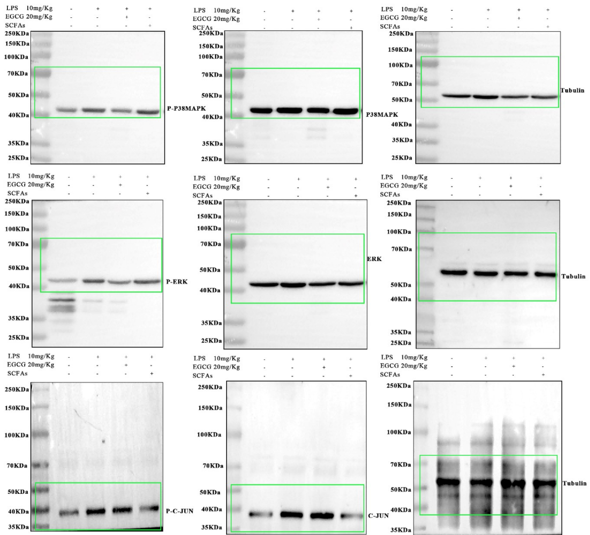
Fig S7.G Full membrane diagramGroup 1
