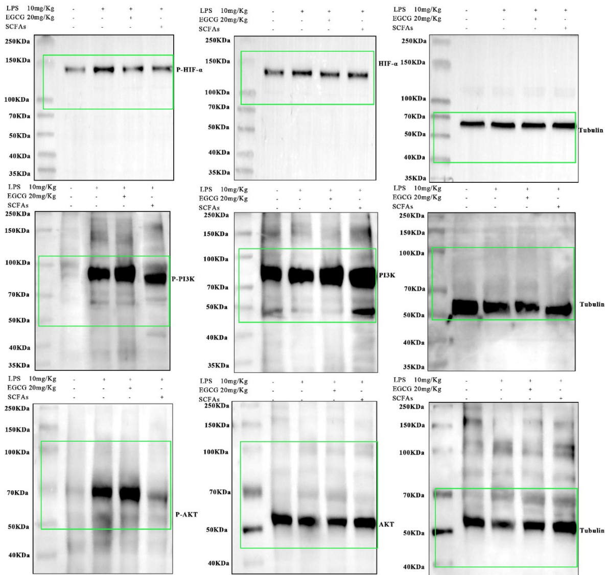
Fig S8.A Full membrane diagramGroup 2
