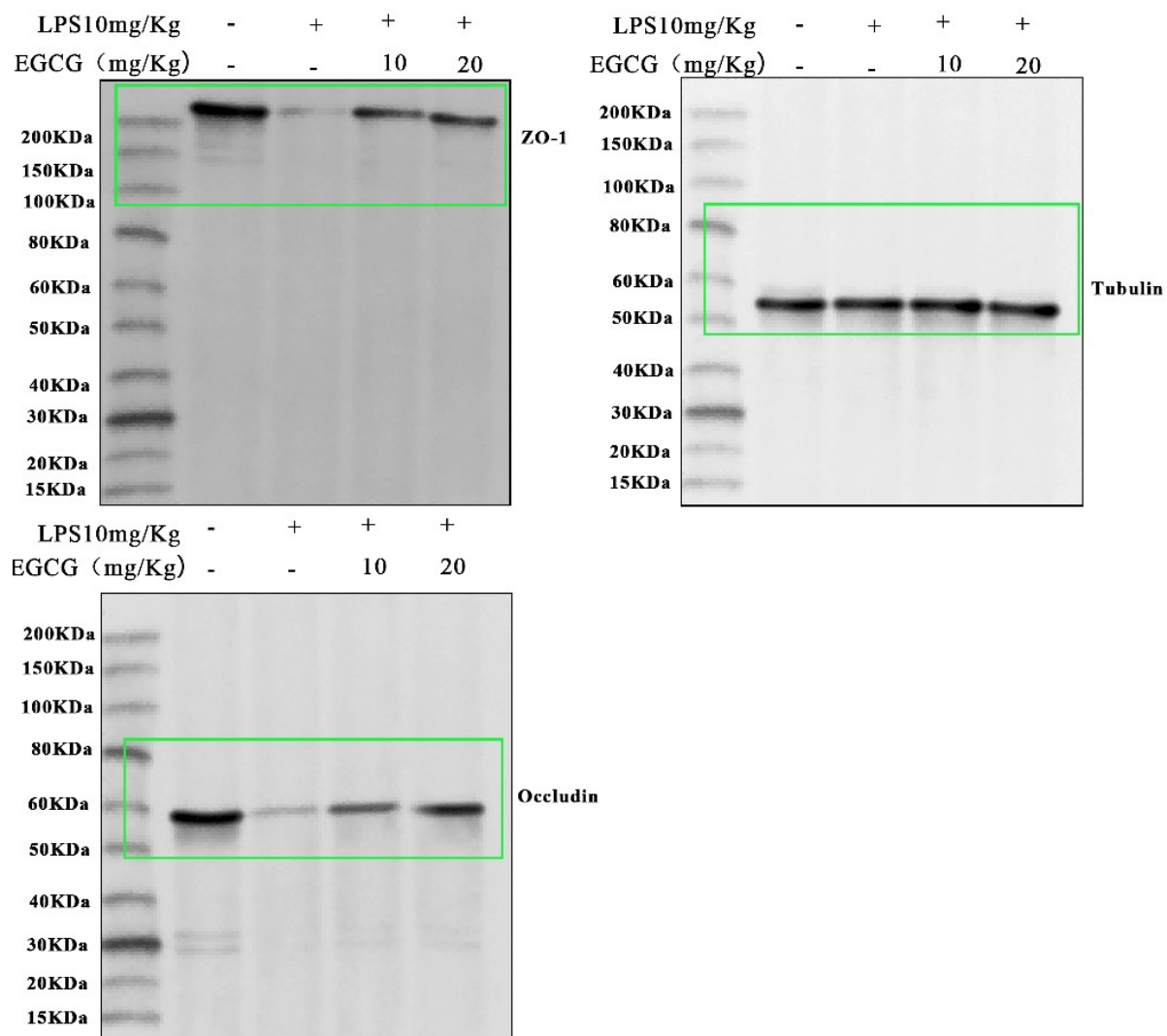
Fig 4.E Full membrane diagramGroup 2
