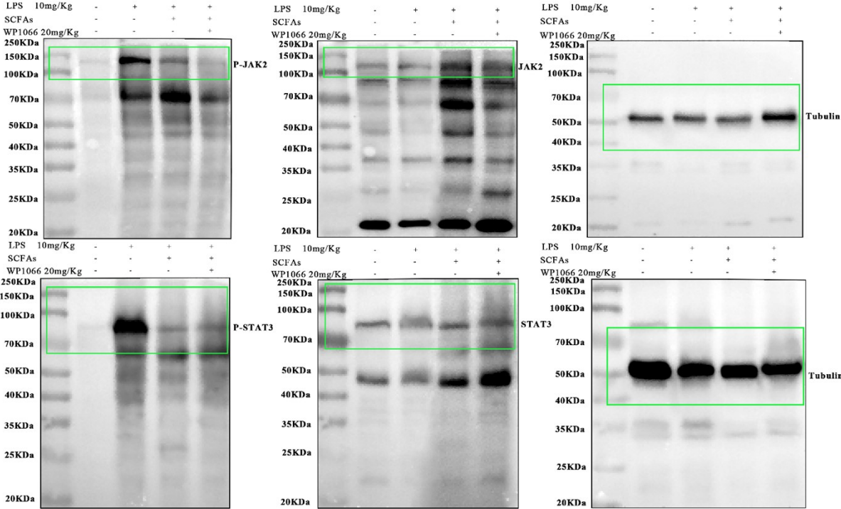
Fig 13.B Full membrane diagramGroup 3
