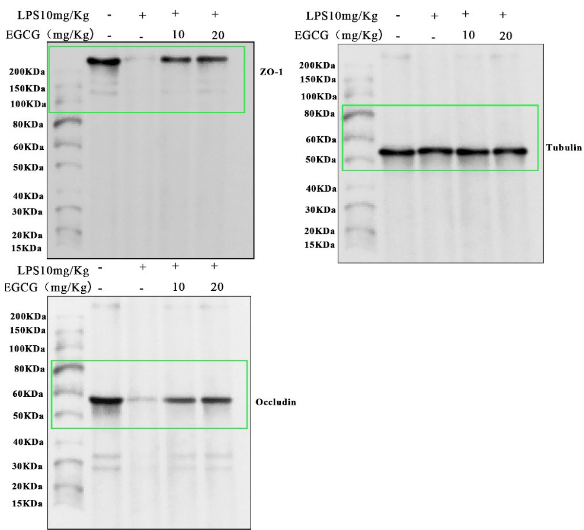
Fig 4.E Full membrane diagramGroup 1
