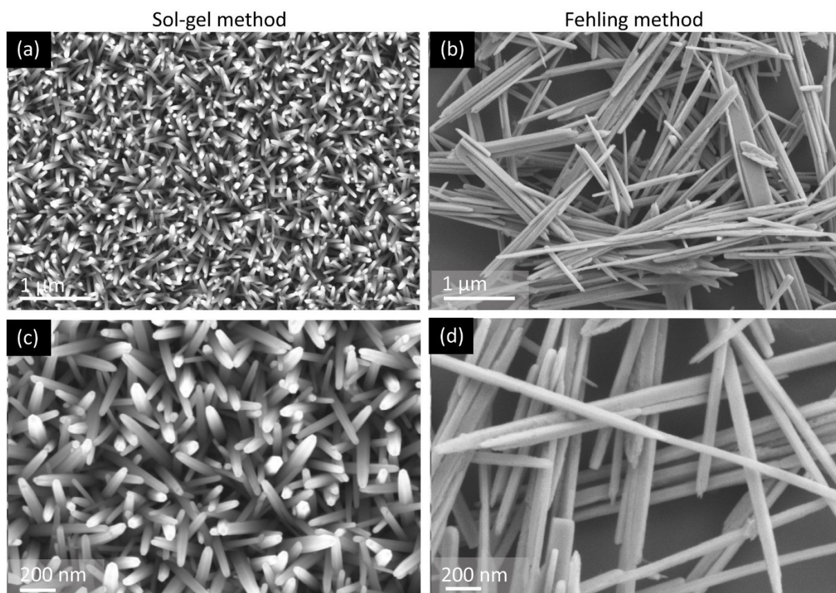
Figure S1: SEM images of ZnO nanowires synthesized by the sol-gel/CBD method (a, c) and the in-solution method inspired by Fehling's reaction (b, d).
