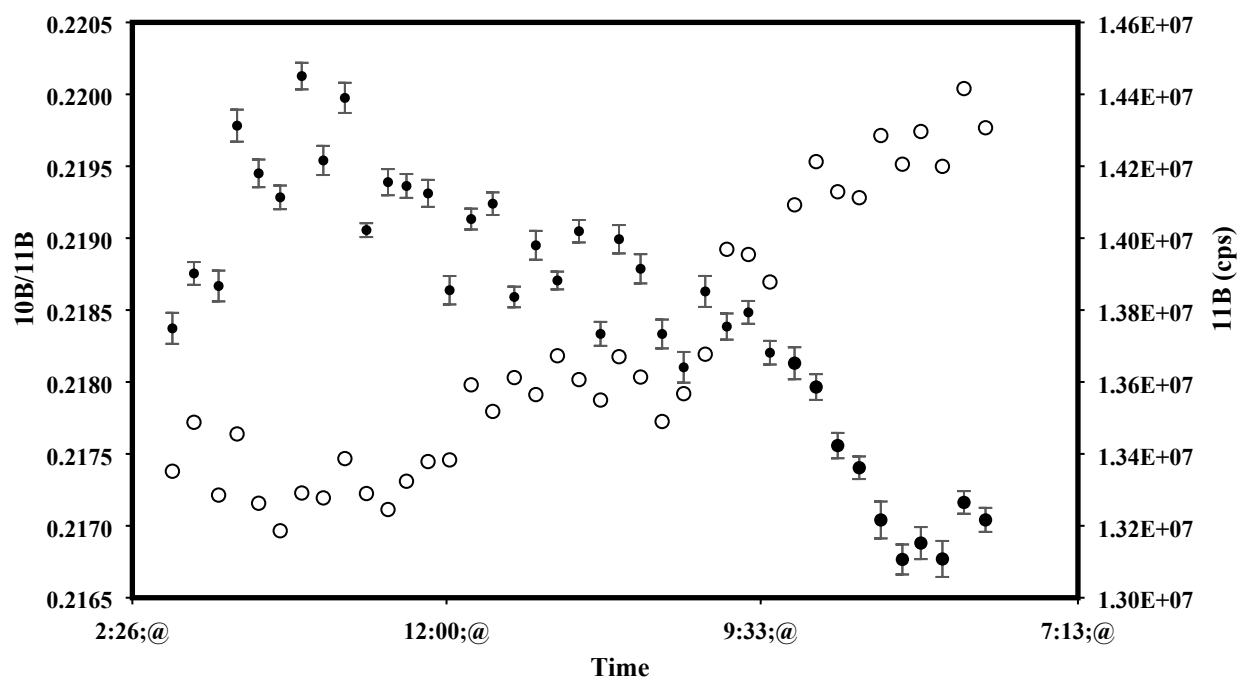
Supplementary Figure 2. Session 4 boron isotopic analysis
