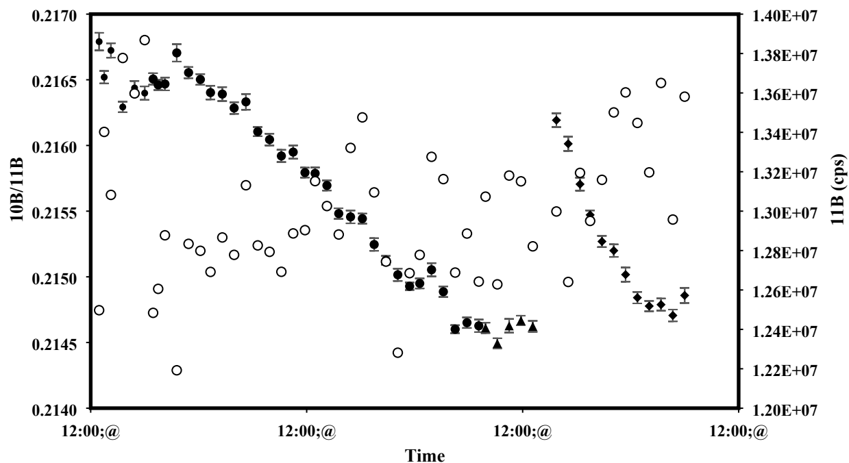
Supplementary Figure 1. Session 3 of boron isotopic analysis
