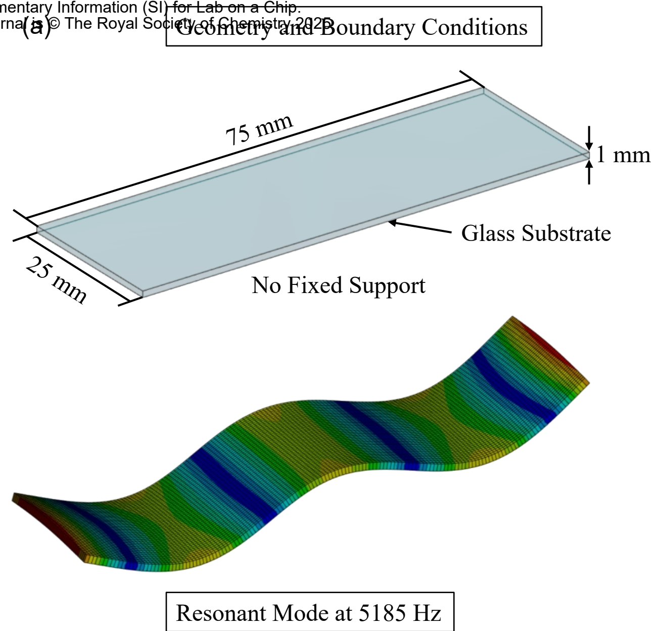
Supplementary 2: Modal analysis results for simplified geometry to represent (a) the glass substrate on its own or (b) substrate with bonded PDMS membrane and channel casting showing 3 rd order lengthwise oscillation modes in the 4-6 kHz range used for actuation in experiments and corresponding membrane oscillation in the free-hanging area.
