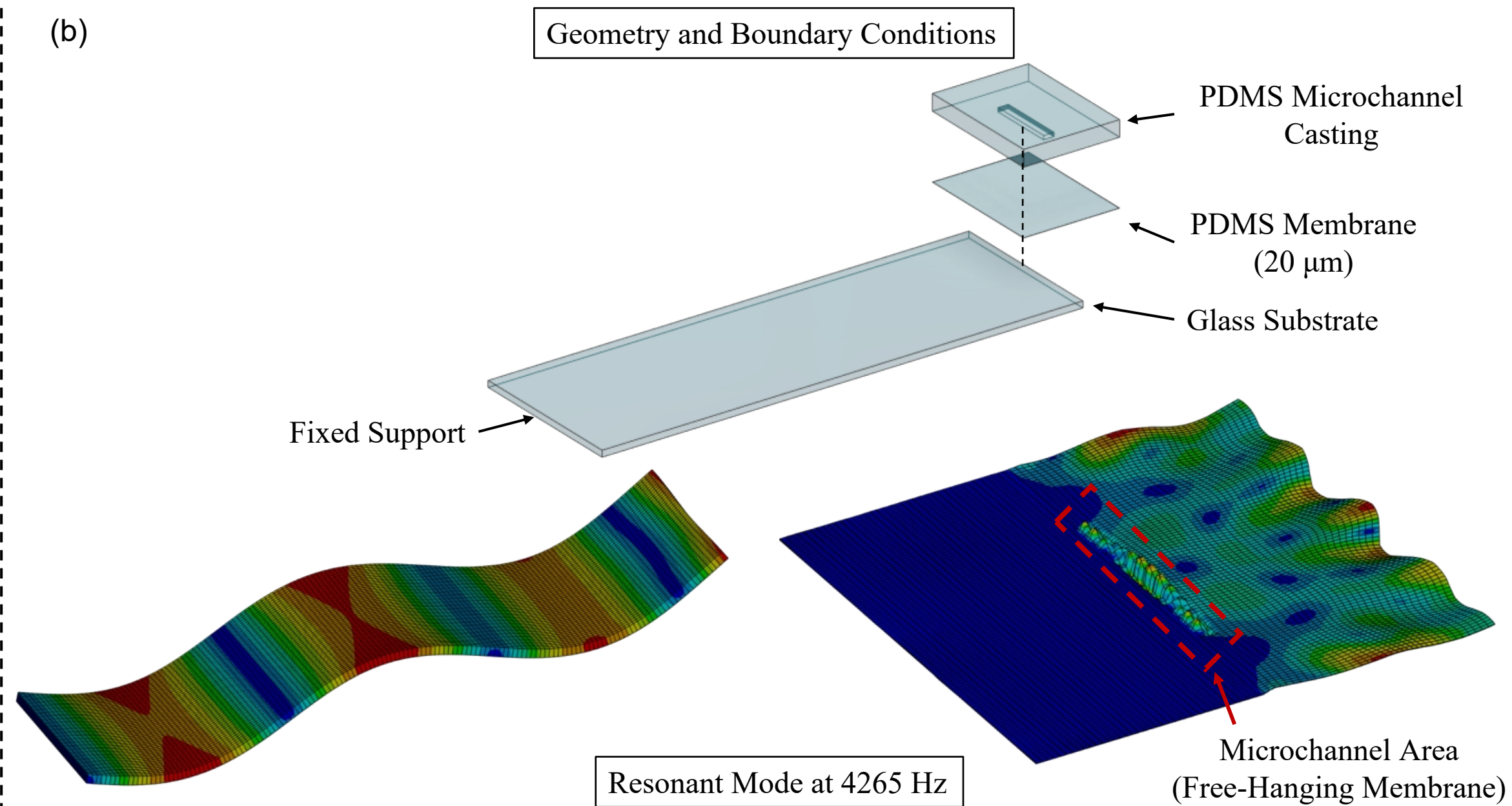
Supplementary 2: Modal analysis results for simplified geometry to represent (a) the glass substrate on its own or (b) substrate with bonded PDMS membrane and channel casting showing 3 rd order lengthwise oscillation modes in the 4-6 kHz range used for actuation in experiments and corresponding membrane oscillation in the free-hanging area.
