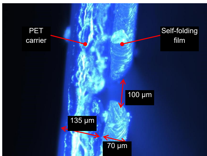
Supplementary Figure S1. Cross-sectional view of laser engraver cutting profile. The cut-width (kerf) is about 100 μm. The cut-depth is about 70 μm.
