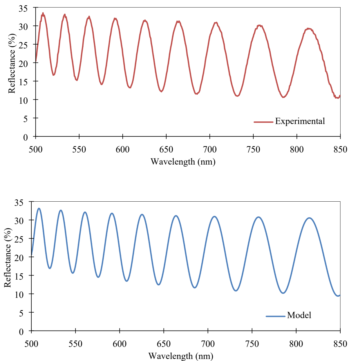
Reflectance vs Wavelength experimental and modeled curve for the 1% wt/wt PMMA at 30%RH
