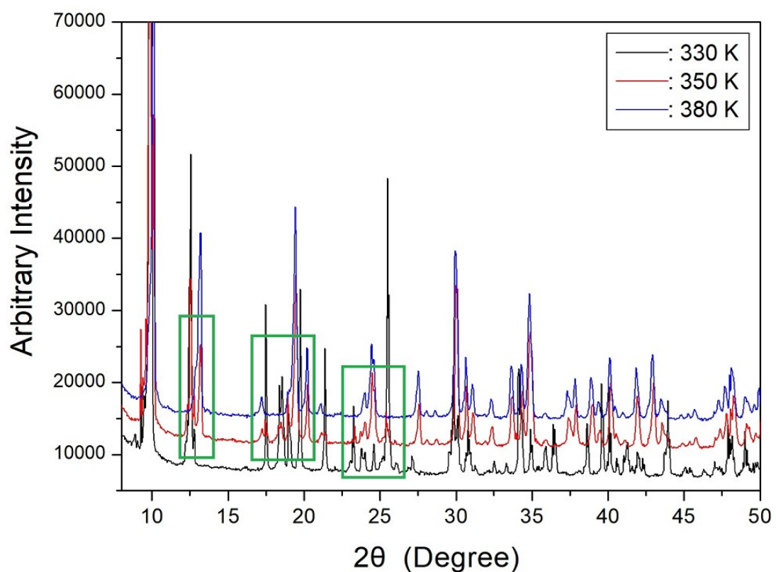
Figure. Powder X-ray diffraction patterns of (\text{CH}_3)_2\text{CHNH}_3\text{CuCl}_3 at 330, 350, and 380 K near phase transition temperature.
