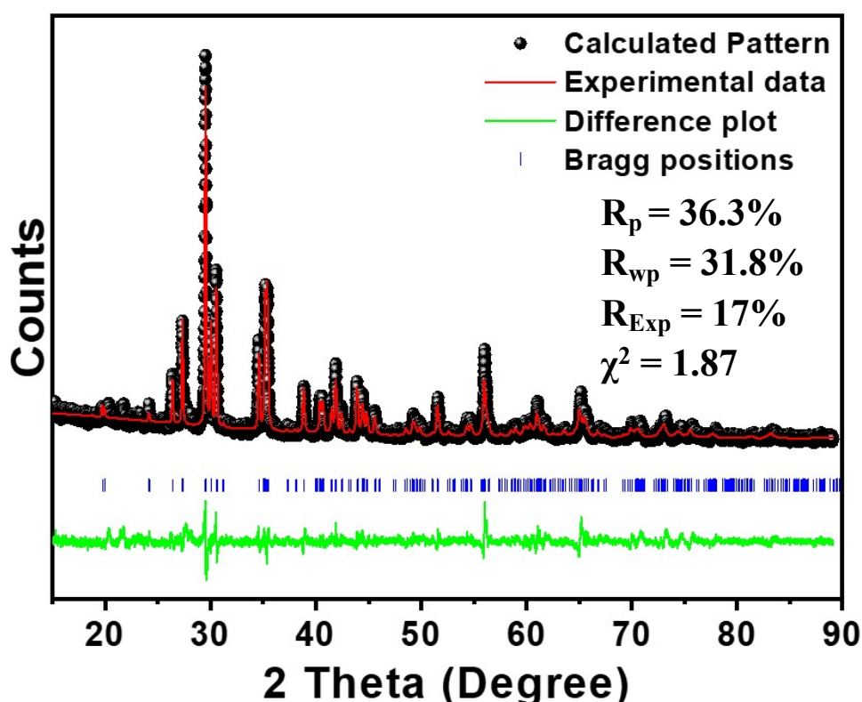
Figure S1: Rietveld refinement analysis of \text{CaMgSi}_2\text{O}_6:0.05\text{Gd}^{3+}
