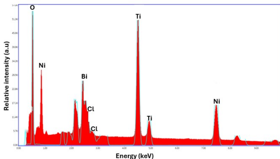
Figure S1: EDX spectra of BiOCl/NiTiO 3 heterostructured semiconductor.
