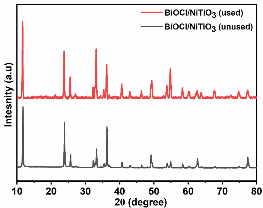
Figure S3: XRD pattern of the \text{BiOCl}/\text{NiTiO}_3 heterostructured semiconductor before and after use in photoelectrocatalytic degradation of CPX
