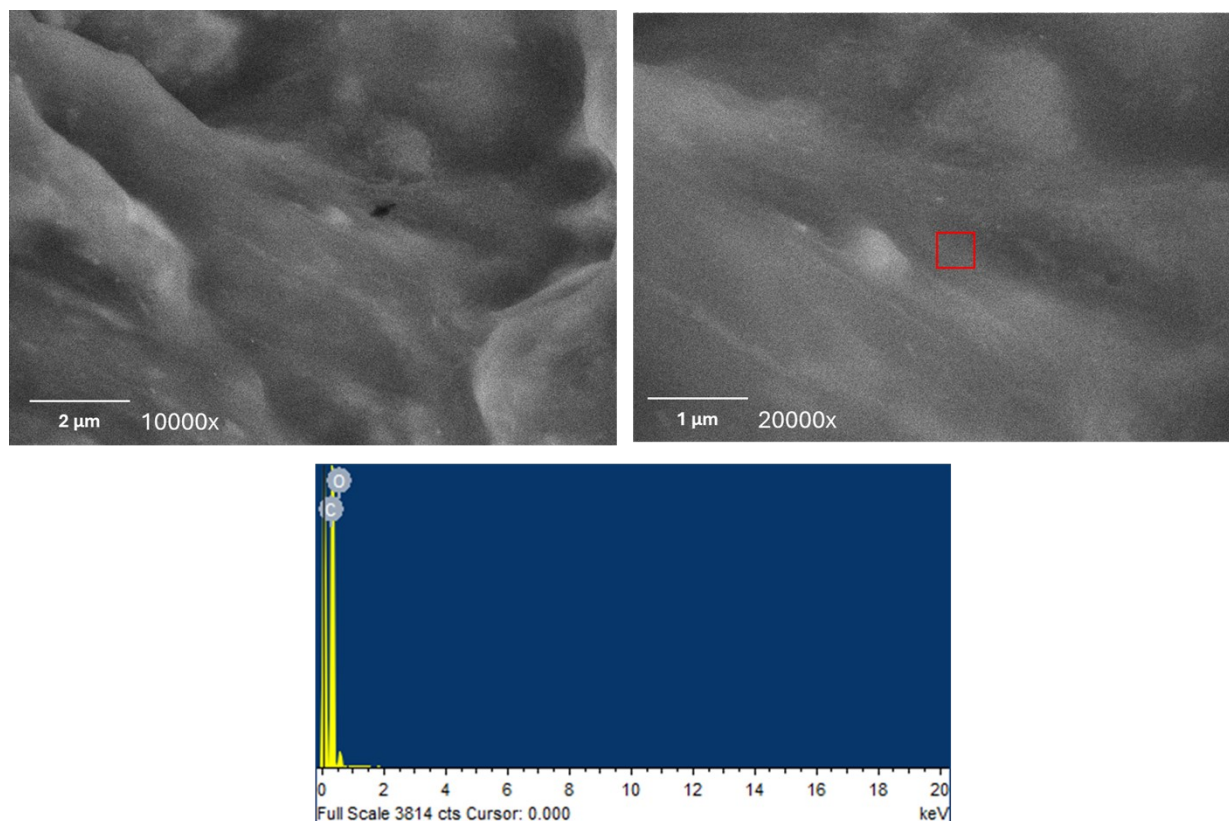
Figure S1: E-SEM images of sample N after drying with EDS on area marked in red.
