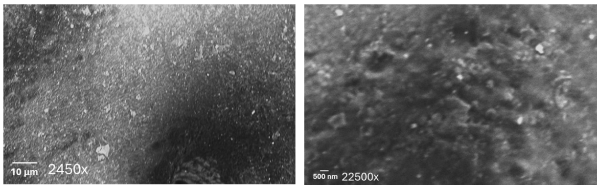
Figure S2: E-SEM images of sample 2.5-LNC after drying.
