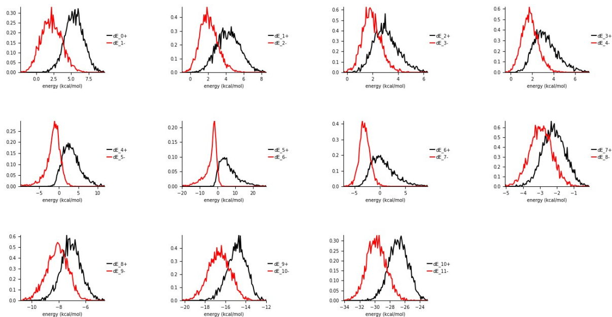
Figure S2: Representative image of overlap of work distributions for transformation with “poor overlap”
