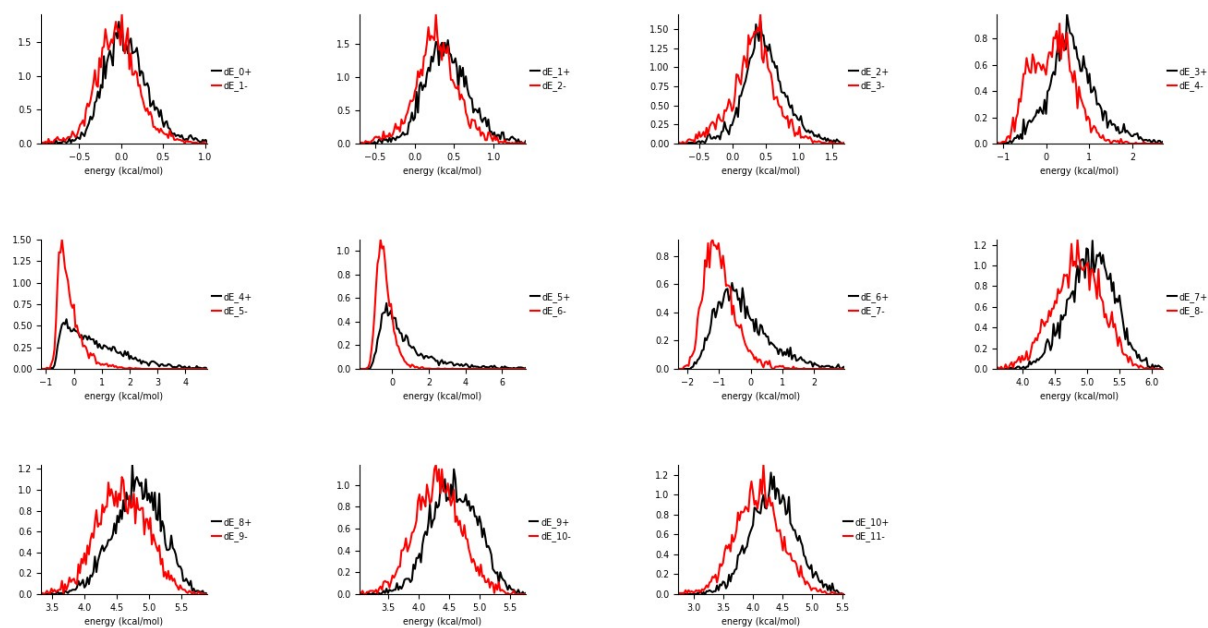
Figure S1: Representative image of overlap of work distributions for transformation with “good overlap”
