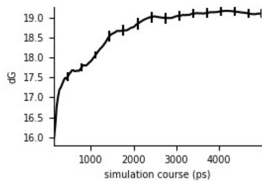
Figure S3: Overall free energy difference (dG) as a function of time of a transformation showing convergence
