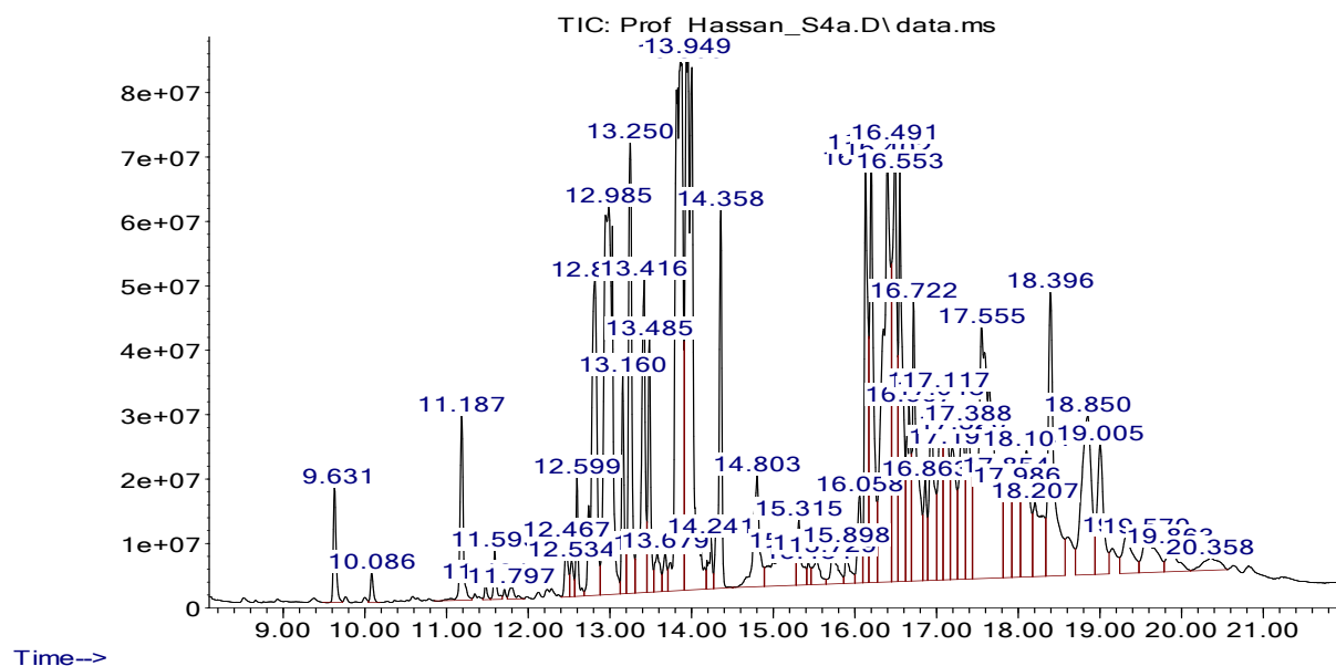
Figure S1. GC-MS Chromatogram for MO extract.
