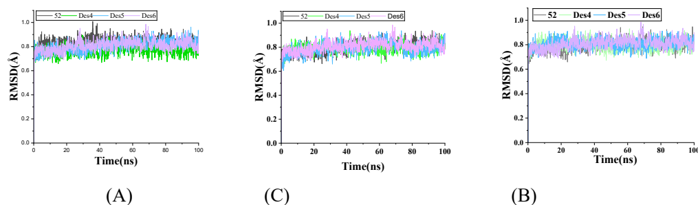
Figure S1. RMSD complexes docked with compound 52/ Des4/ Des5/ Des6 for 100 ns simulations((A): The first time (B) : The second time(C) : The third time).
