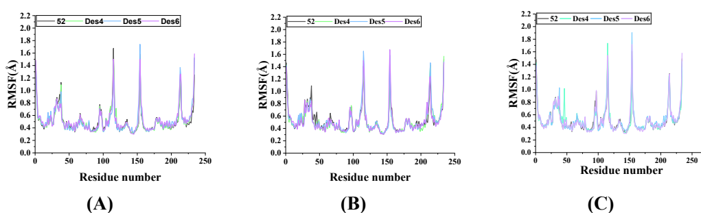
Figure S2. RMSF complexes docked with compound 52/ Des4/ Des5/ Des6 for 100 ns simulations((A): The first time (B) : The second time(C) : The third time).
