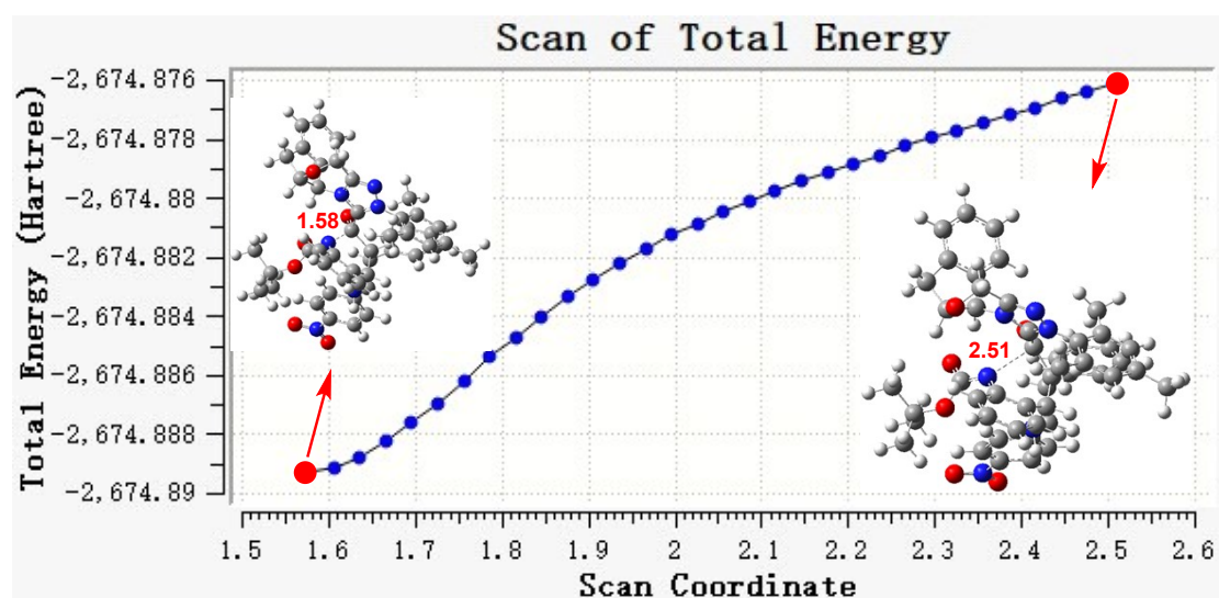
Fig. S4 Scanning results of SR -configured pathway involved in the lactamization process
