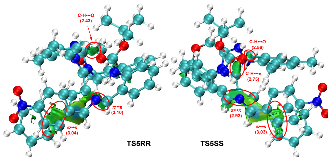
Fig. S5 NCI analysis for stereoselective transition states TS5RR and TS5SS (distances are given in Å)
