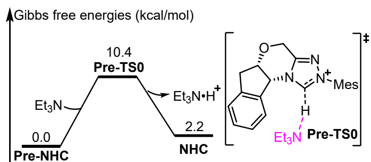
Fig. S1 Relative Gibbs free energy profile for the formation of NHC
