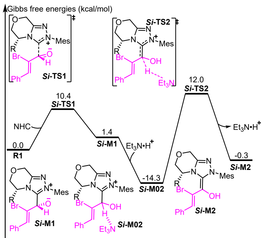
Fig. S2 Relative Gibbs free energy profile for the formation of Breslow intermediate via the Si-face addition mode
