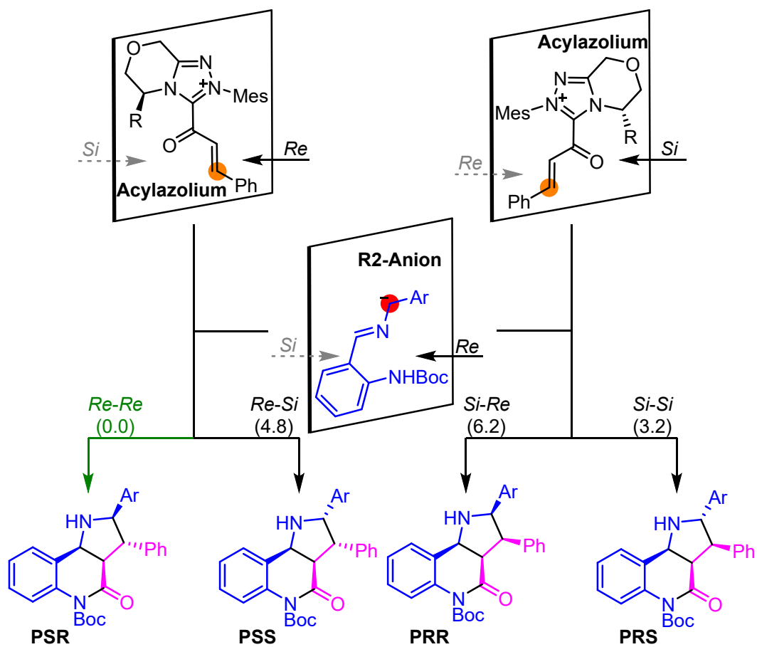
Scheme S1. Possible stereoselective addition modes
