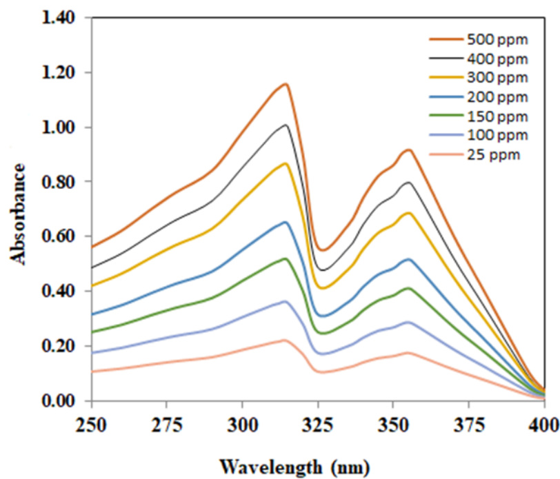
Figure S1. The UV absorbance vs. CBZ concentrations in the range of 250 to 400 nm.
