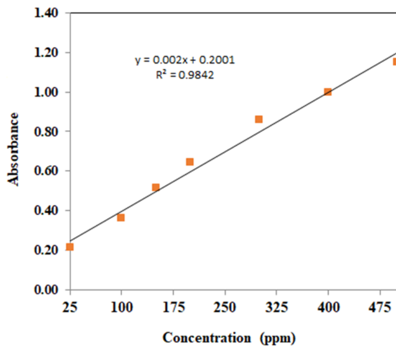
Figure S2. Calibration curve of absorbance versus CBZ concentration for the peak at 315 nm.
