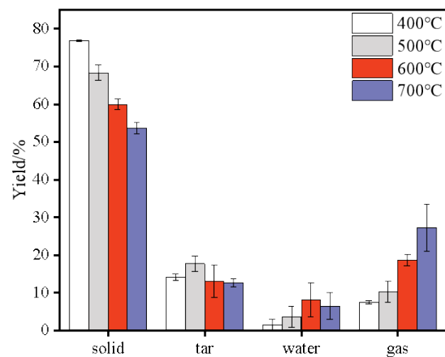
Fig. 1. Product distribution at different pyrolysis temperatures
