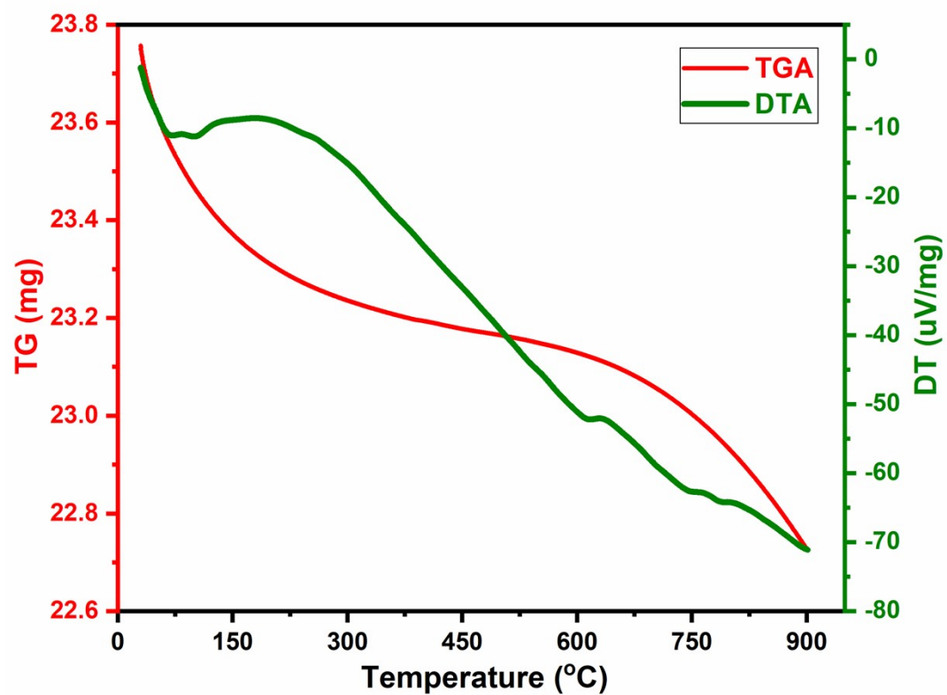
Figure S1: TGA-DTA Analysis of \text{Sr}_6\text{Ca}_4(\text{PO}_4)_6\text{F}_2 phosphor.
