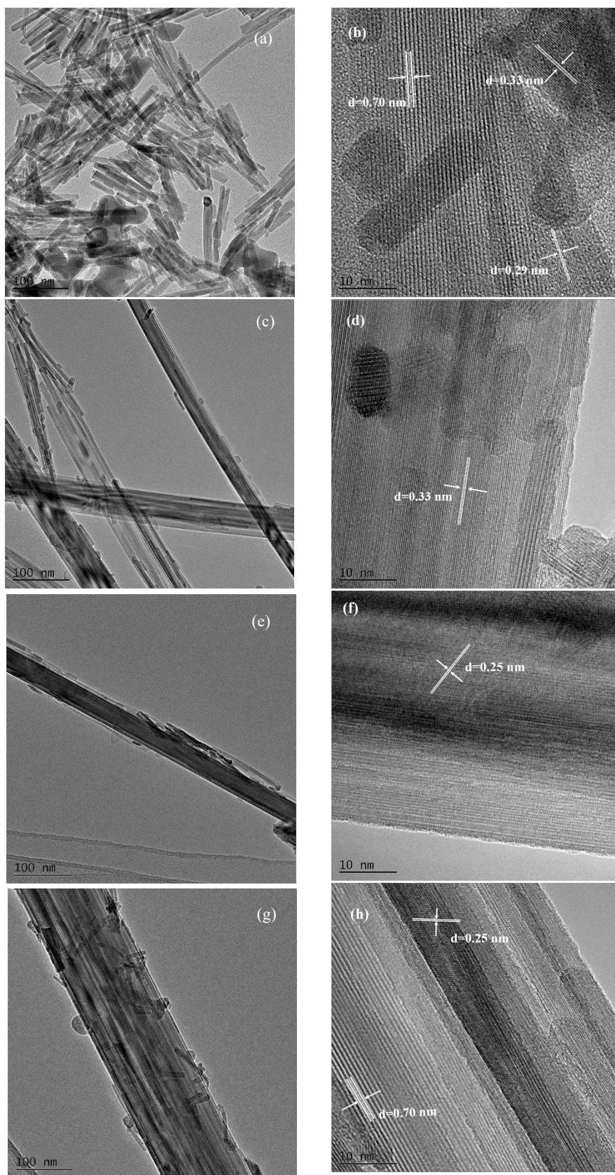
Fig. S2 TEM image of the samples: a-b: Ag/OMS-R, c-d: Ag/OMS-E, e-f: Ag/OMS-I (c) and g-h: OMS
