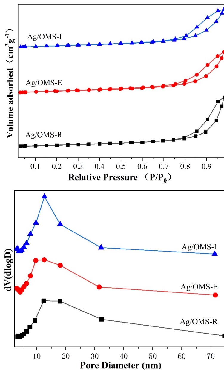
Fig. S1 N_2 adsorption/desorption isotherms and pore-size distribution of catalysts.
