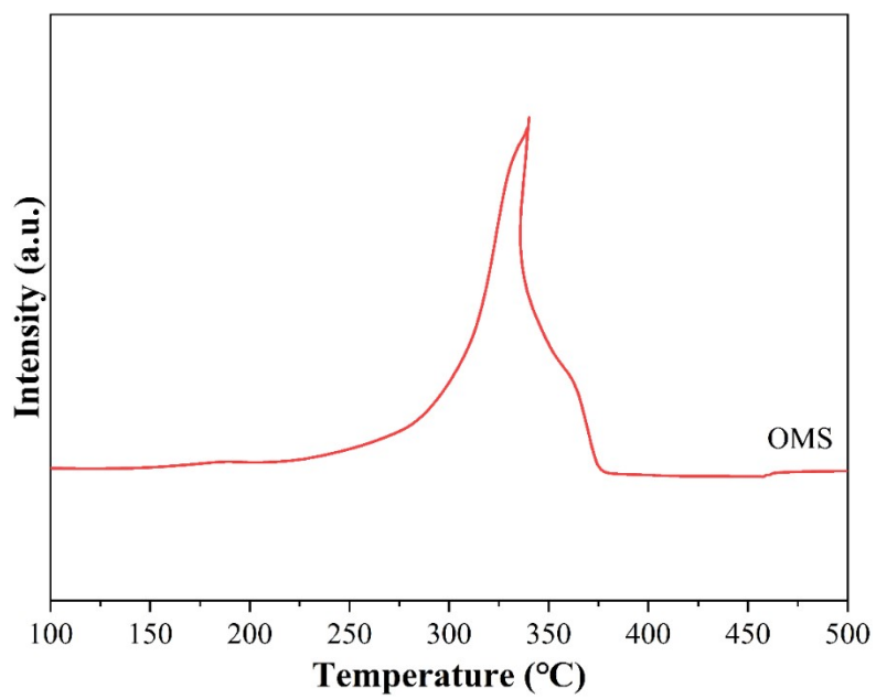
Fig. S3 TPR result of OMS sample
