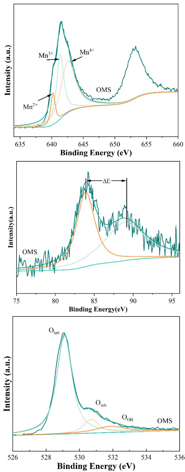
Fig. S4 XPS results of OMS sample
