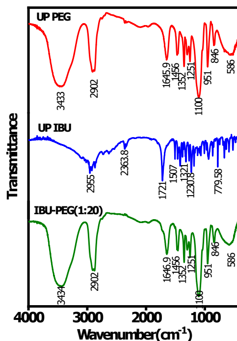
Fig S2. FT-IR spectrum of unprocessed IBU, unprocessed PEG, and scCO 2 -processed IBU-PEG.
