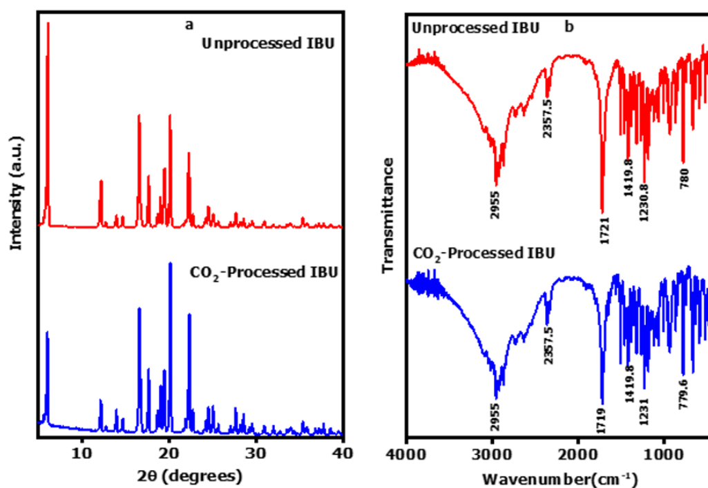
Fig S1. (a) XRD pattern of IBU before and after scCO 2 processing; (b) FT-IR spectrum of IBU before and after scCO 2 processing.
