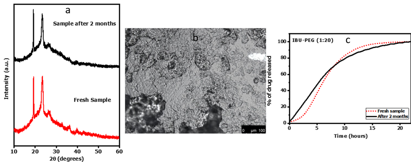
Fig S3. (a) XRD pattern of IBPEGCO 2 just after scCO 2 -processing and after two months of storage; (b) optical microscopic image of IBPEGCO 2 after two months; and (c) drug-release curves of IBPEGCO 2 after two months with the reference curve of a fresh sample.
