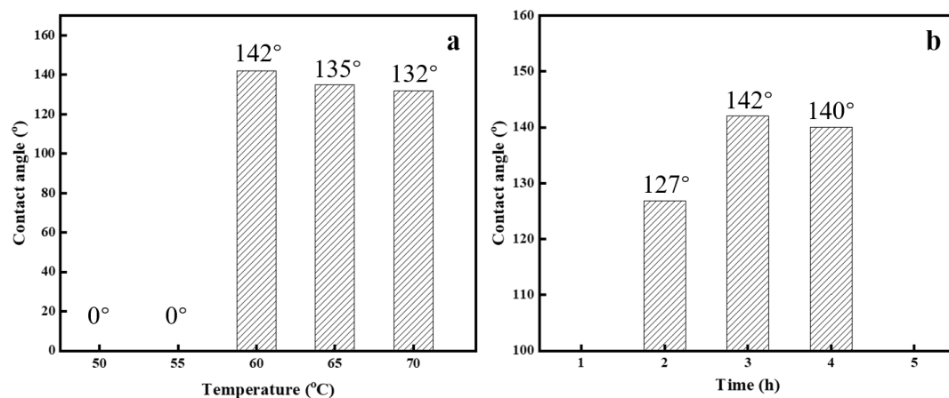
Fig. S1 Effect of grafting reaction temperature (a) and time (b) on the contact angle of GO-g-PBA.
