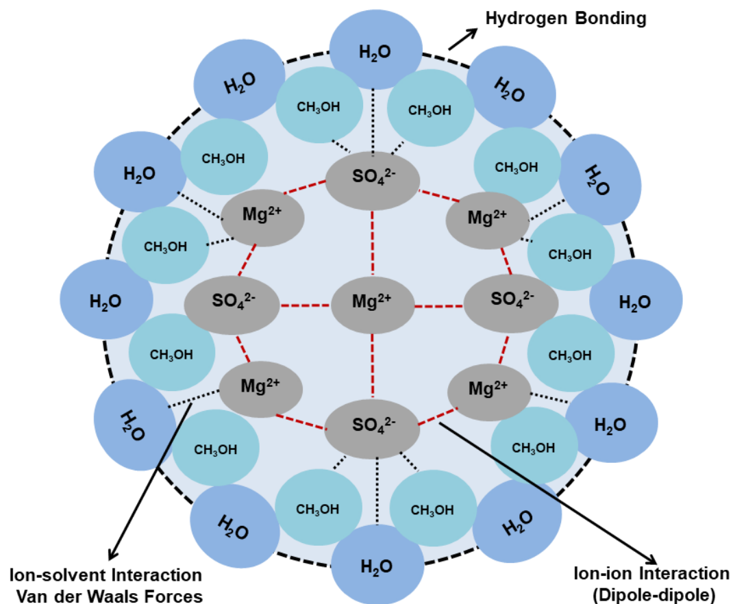
Pictorial Representation of Water-Ethanol-Mg 2+ /SO 4 2- Clusters (Graphical Abstract)
