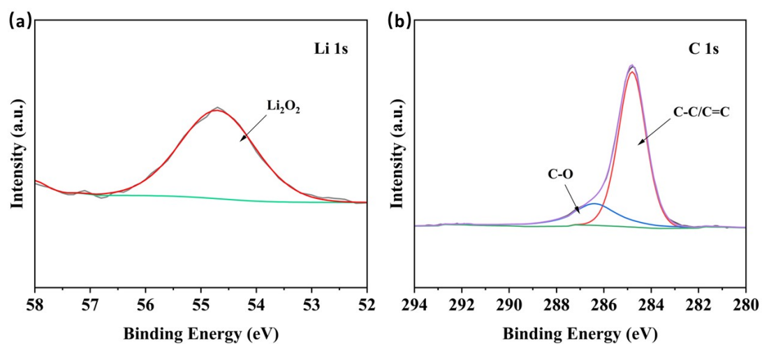
Figure S1 The Li 1s and C 1s spectrum of the discharged PtFeCoNiCu@rGO cathode with a specific capacity of 2000 mAh g -1
