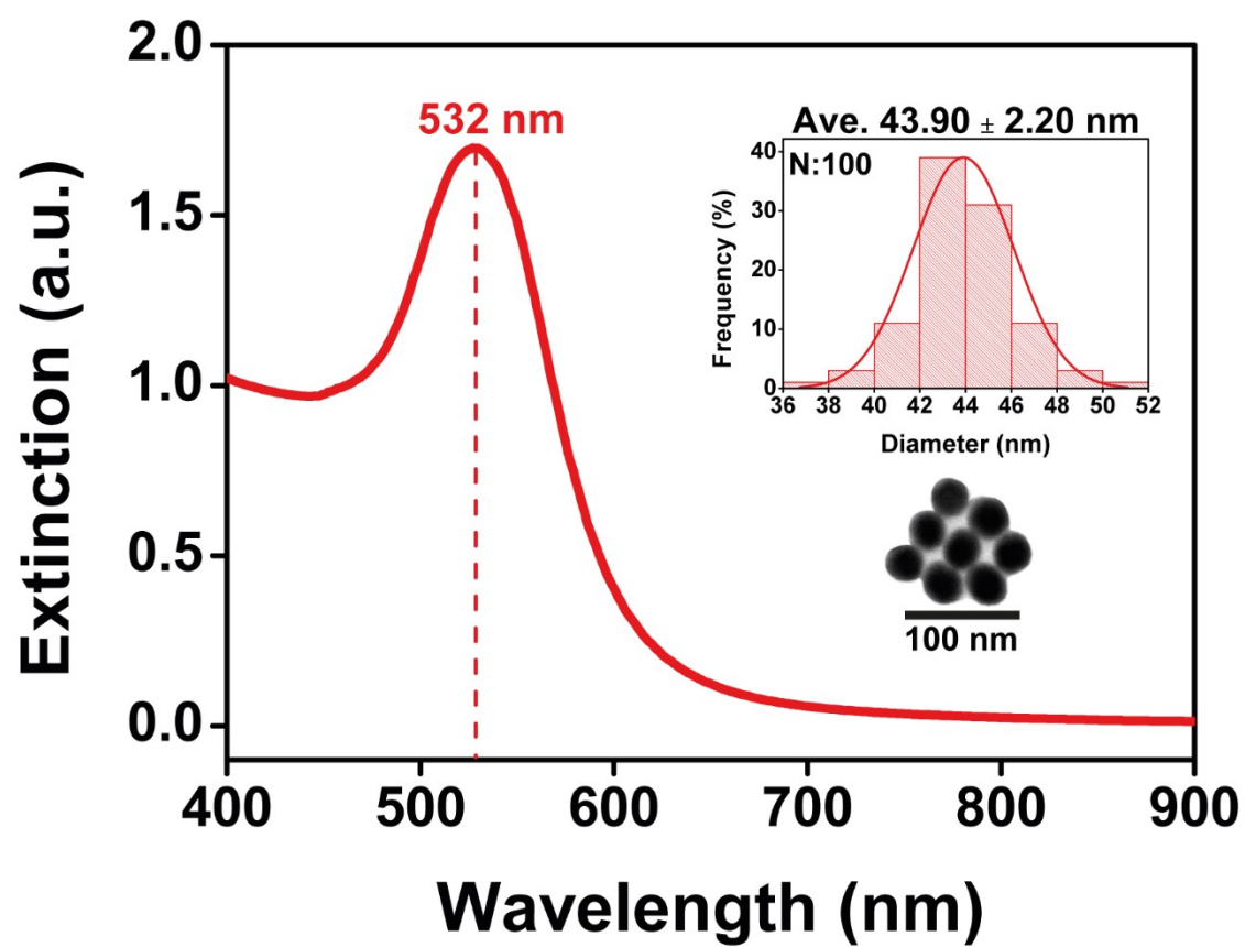
Fig. S1 Characterization of AuNPs by UV-vis spectroscopy and STEM (20.0 kV).
