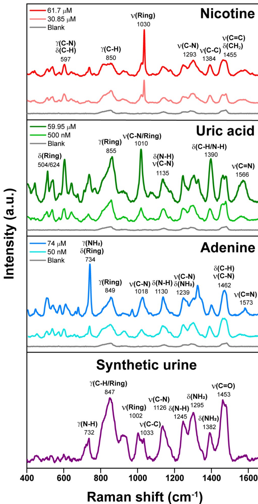
Fig. S7 Detection of bioanalytes and analysis of synthetic urine using the proposed 3D-printed SERS substrates based on AuNPs.
