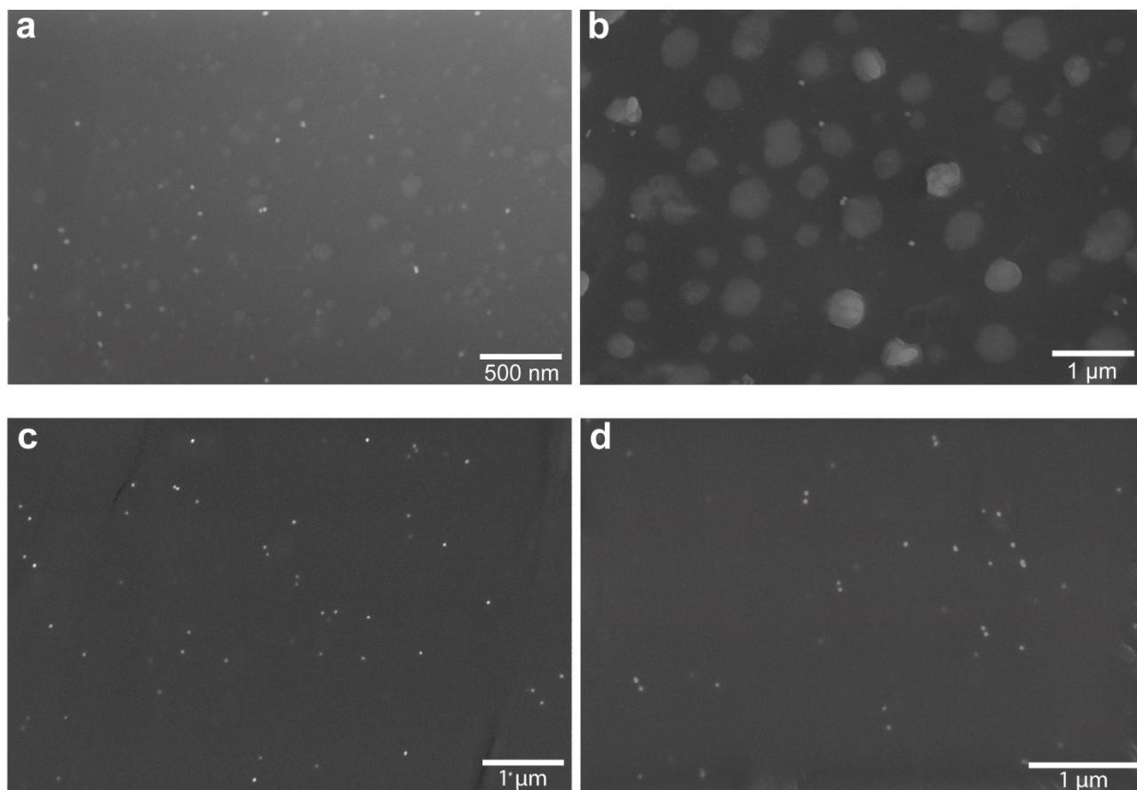
Fig. S6 SEM micrographs in environmental mode (20 kV, 200 Pa) of hydrated (a) AuNPs and (b) AgNPs substrates in environmental mode (20 kV, 200 Pa) and anhydrous (c) AuNPs and (d) AgNPs substrates under high vacuum mode (5 kV).
