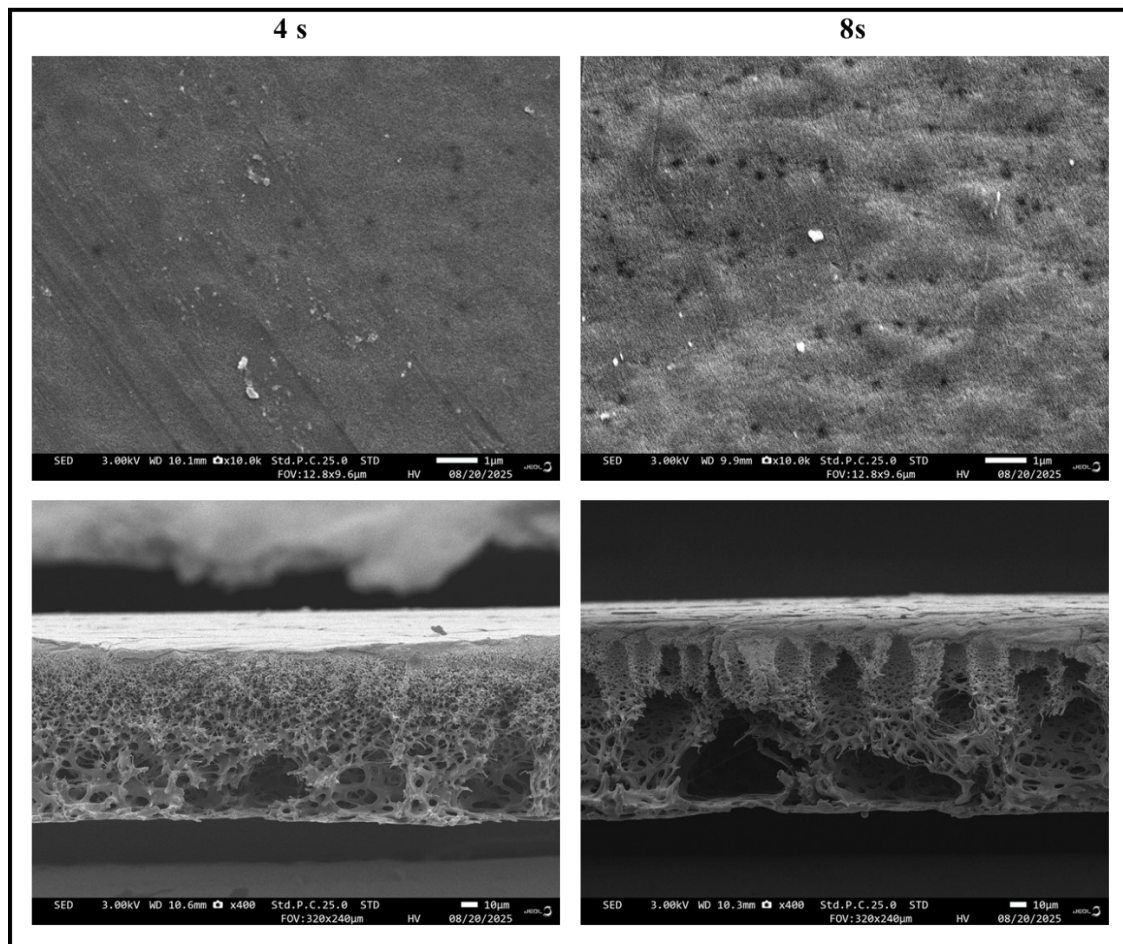
Figure S1: Top surface and cross-sectional SEM images of PES Nanofilms prepared at (a) t_{\text{exp}} = 4 s and (b) 8s. Scale bars: 1 \mu\text{m} (surface) and 10 \mu\text{m} (cross-section).
