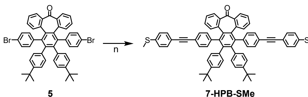
Scheme S4: ( n ) (4-ethynylphenyl)(methyl)sulfane, PdCl 2 (CH 3 CN) 2 , CuI, PtBu 3 ·HBF 4 , THF, i Pr 2 NH, 70 °C, 16 h
