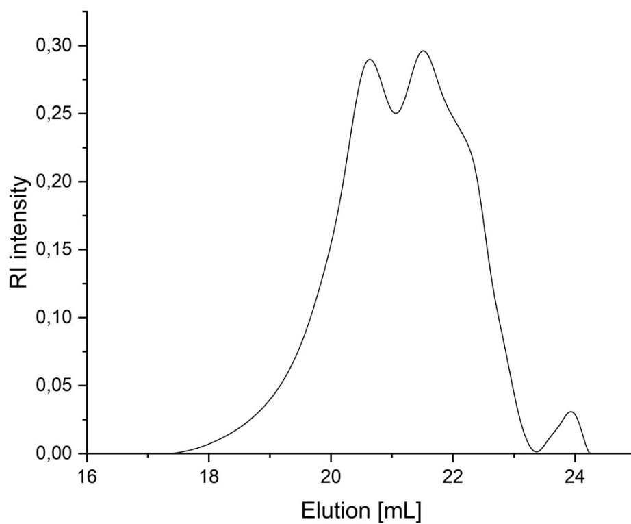
Figure S2 GPC elution curve of PGA No. 7, Table 2
