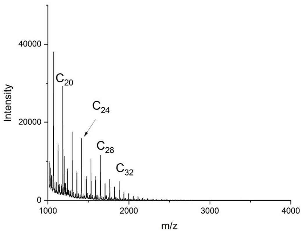
Figure S3 MALDI TOF mass spectrum of PGA No. 9, Table 2
