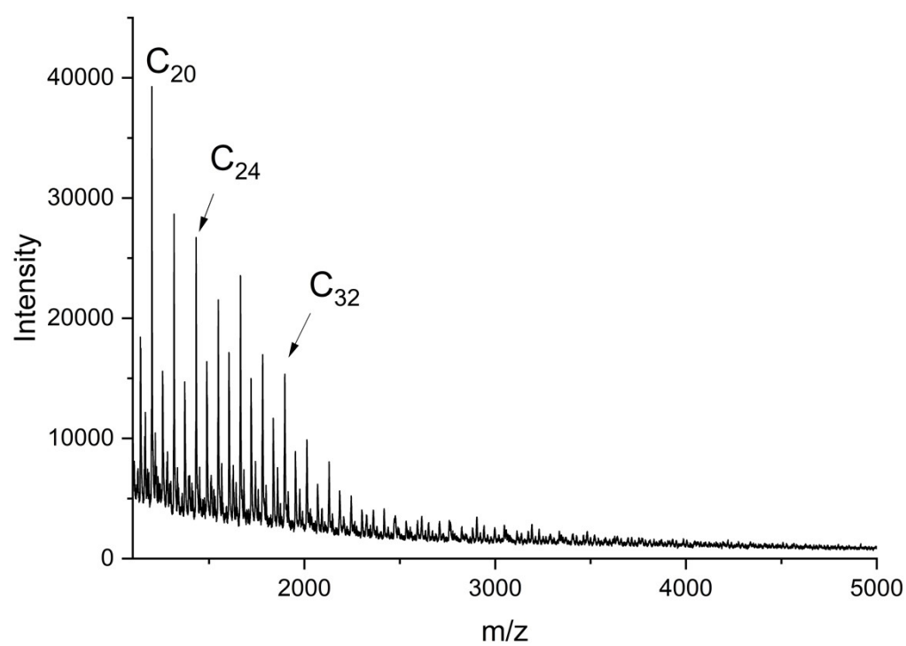
Figure S4 MALDI TOF mass spectrum of PGA No. 11, Table 2
