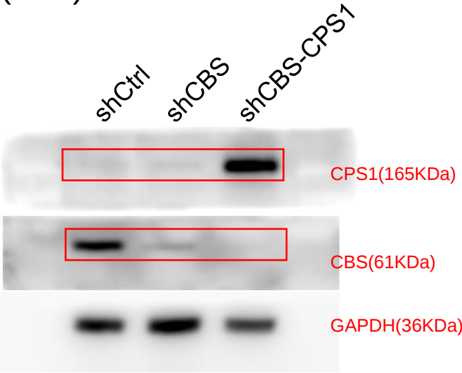
Figure 7F-CBS/CPS1 (N=3)
