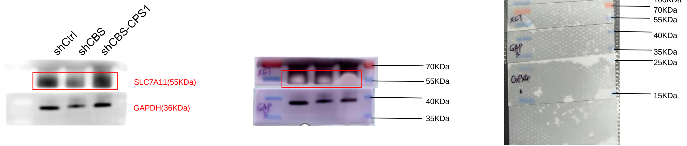
Figure 7F-xCT/SLC7A11
