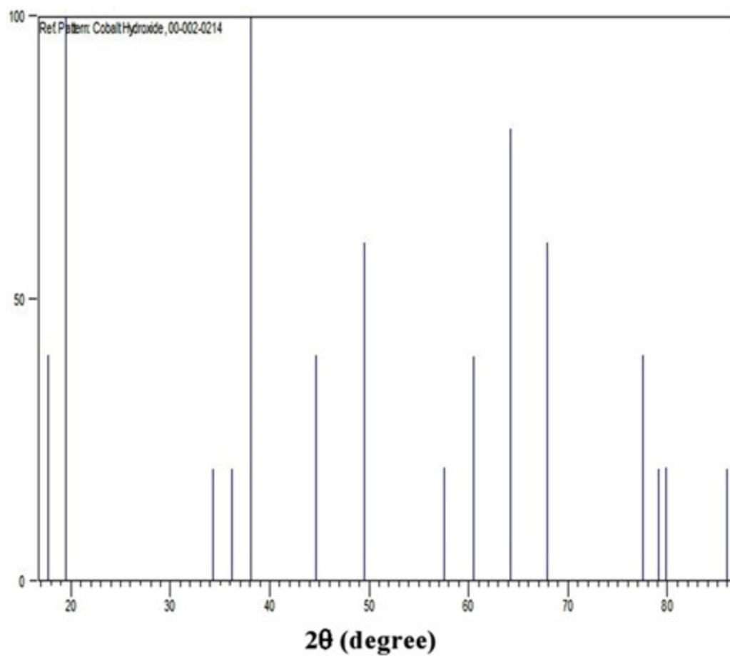
Fig. S2. Reference XRD spectrum of cobalt hydroxide
