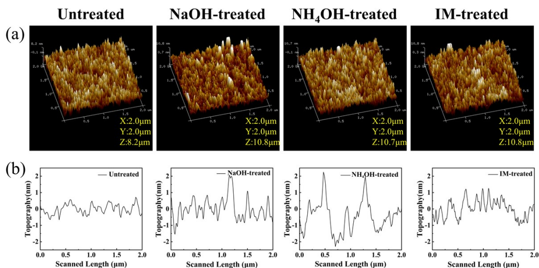
Fig.S3 (a) AFM topography images of PEDOT:PSS films; (b) Surface profiles corresponding to the topography images.
