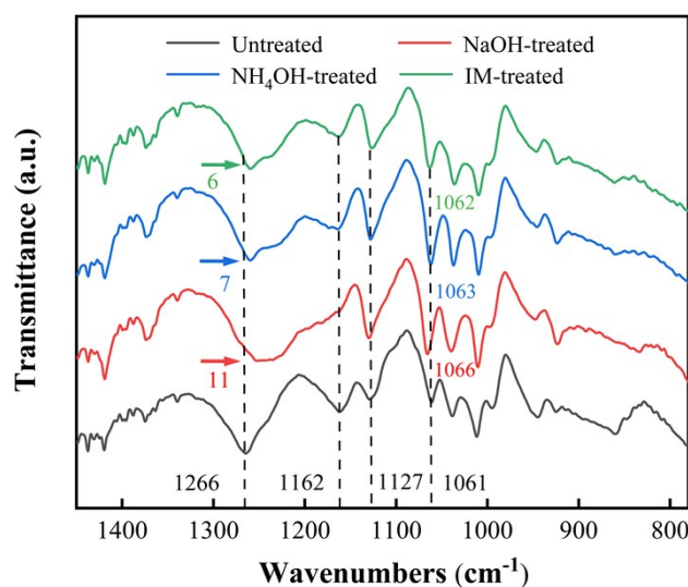
Fig.S1 ATR-FTIR spectra for untreated PEDOT:PSS films and films treated with three bases
