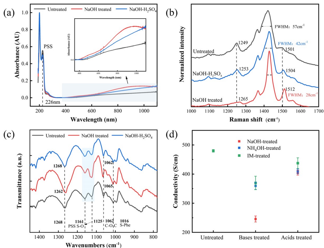
Fig.S2 Doping level characterization and conductivity of PEDOT:PSS films with acid re-treatment after bases treatment. (a) The UV absorption spectra; (b) Raman spectra measured at a 532 nm laser; (c) ATR-FTIR spectra; (d) conductivity of PEDOT:PSS films.
