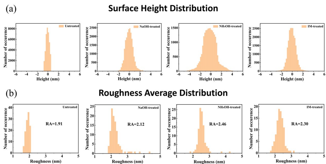
Fig.S4 (a) Surface height distribution corresponding to the images; (b) Surface roughness distribution of the films.
