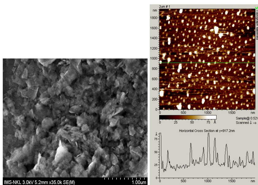
Fig. S2. SEM and AFM images of hBN flakes
