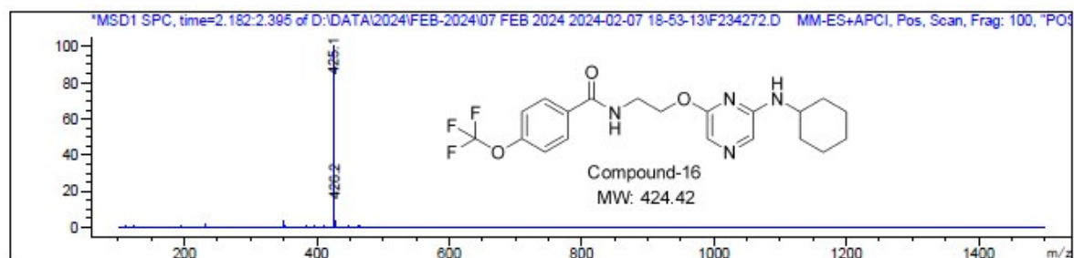
1 H & 13 C-NMR and MS-Spectrum of compound-17a
