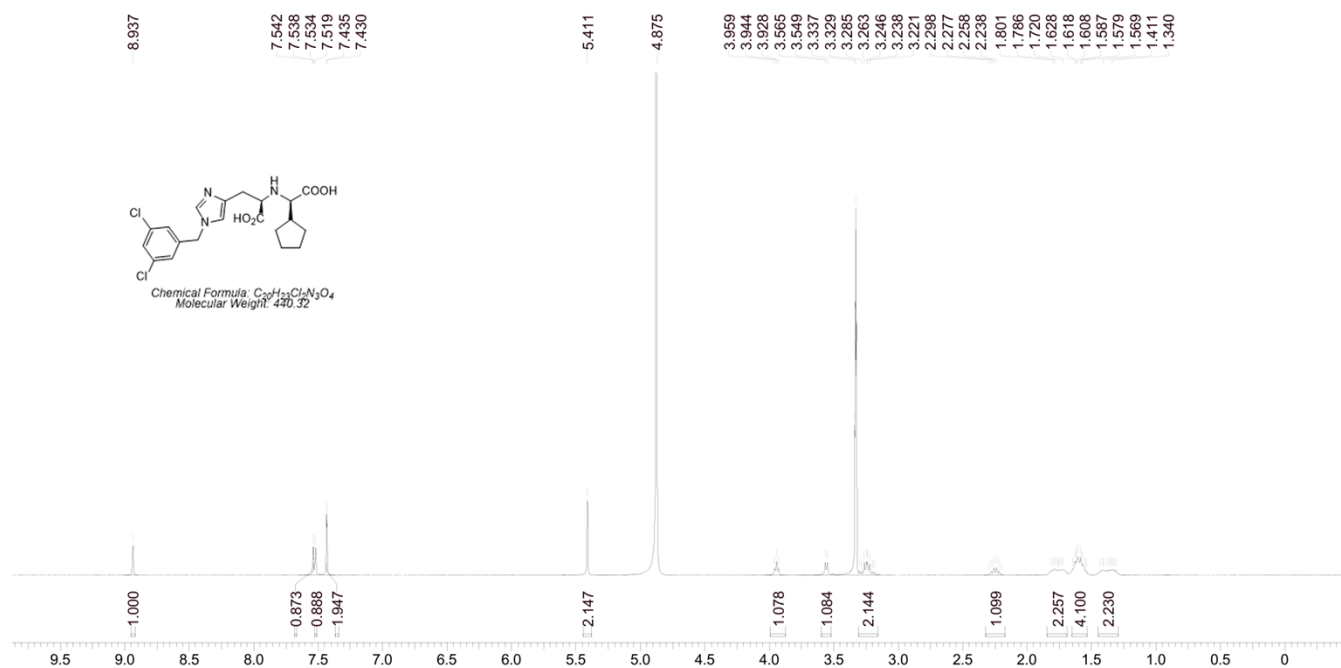
Supplement 1 Figure 1. ^1\text{H} -NMR for LMS1007
