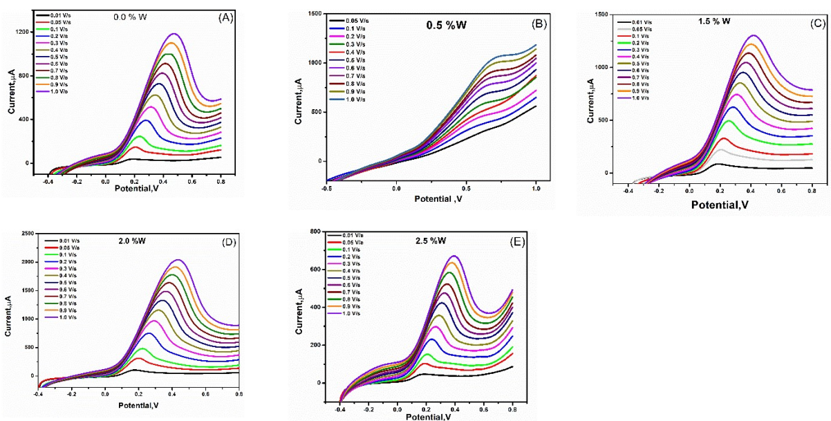
Figure 1S : (A-E) LSVs curves for synthesized CdO-ZnO-W-P 2 O 5 (CZWP) with different % of tungsten (A) 0.0 %W , (B) 0.5 %W, (C) 1.5 %W , (D) 2.0 %W and (E) 2.5 %W modified SPEs at different scan rates
