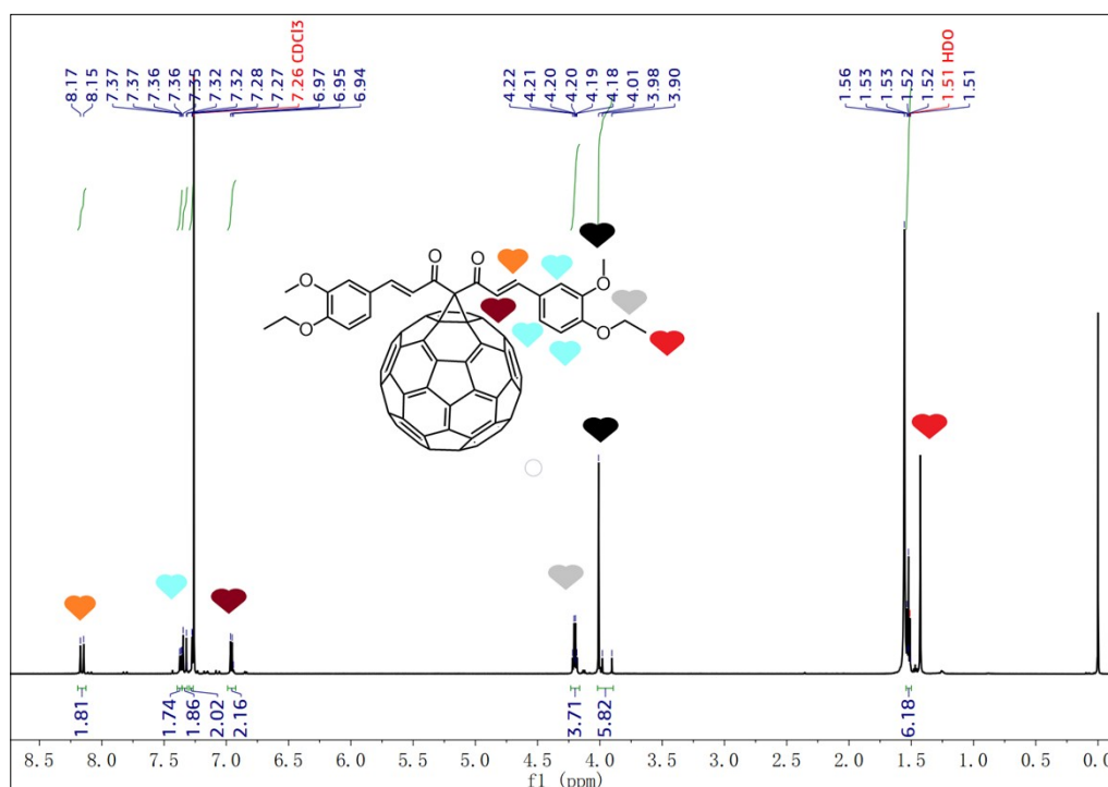
Fig. S1 1 H NMR spectra of compound 2a
