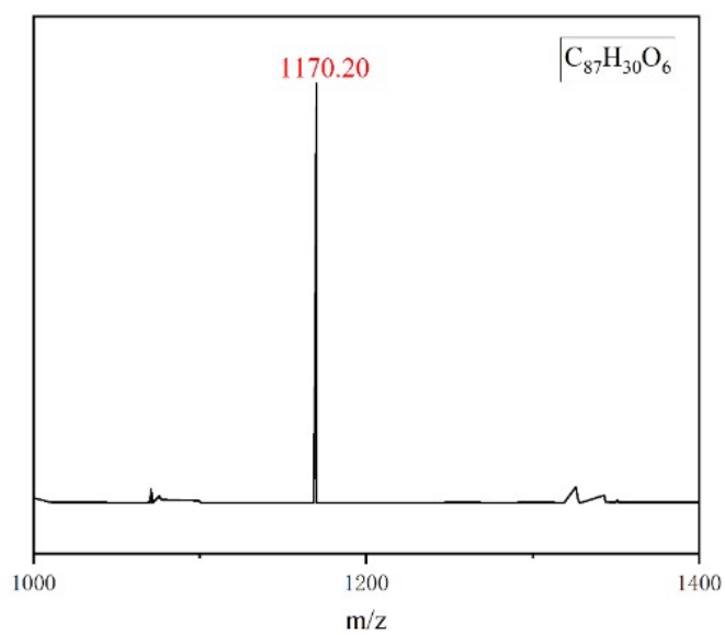
Fig. S6 HRMS of compound 2b
