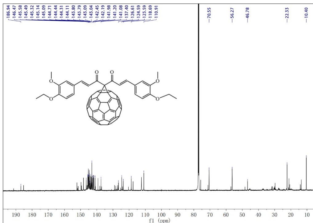
Fig. S2 13 C NMR spectra of compound 2a
