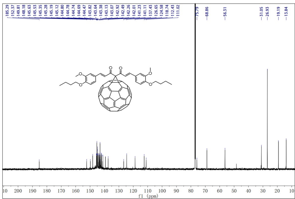
Fig. S8 13 C NMR spectra of compound 2c
