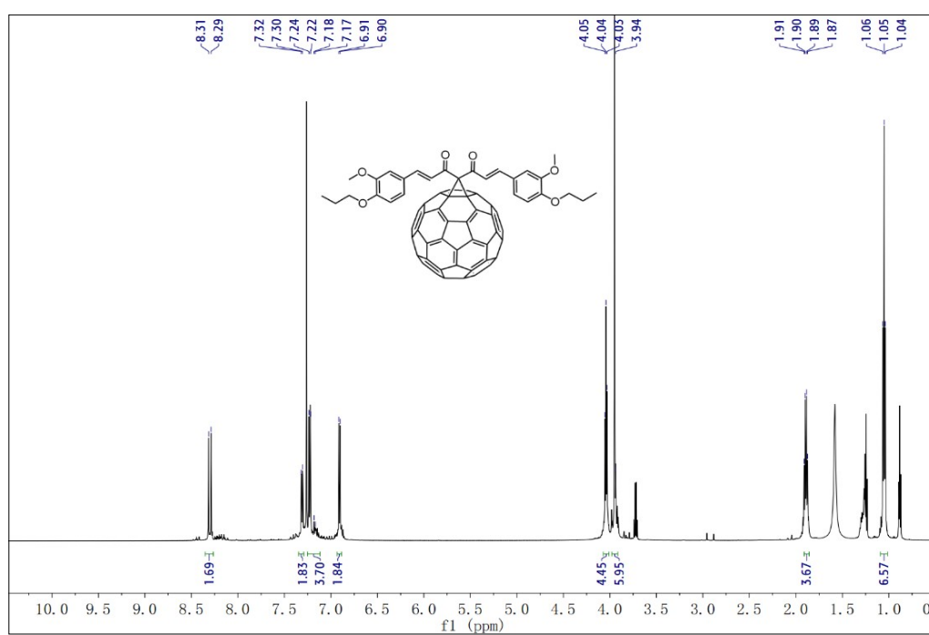
Fig. S4 ^1H NMR spectra of compound 2b
