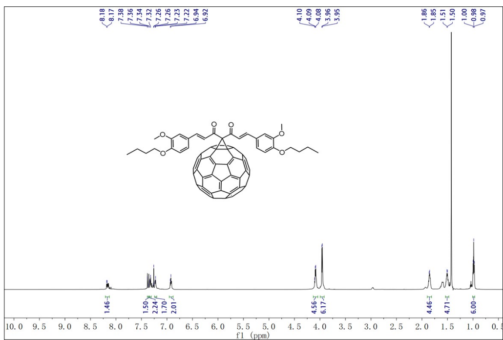
Fig. S7 1 H NMR spectra of compound 2c
