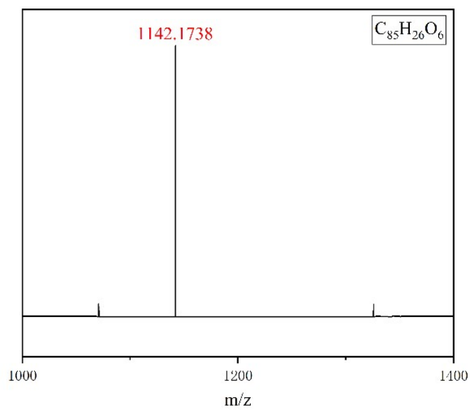
Fig. S3 HRMS of compound 2a
