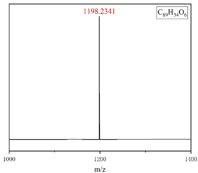
Fig. S9 HRMS of compound 2c
