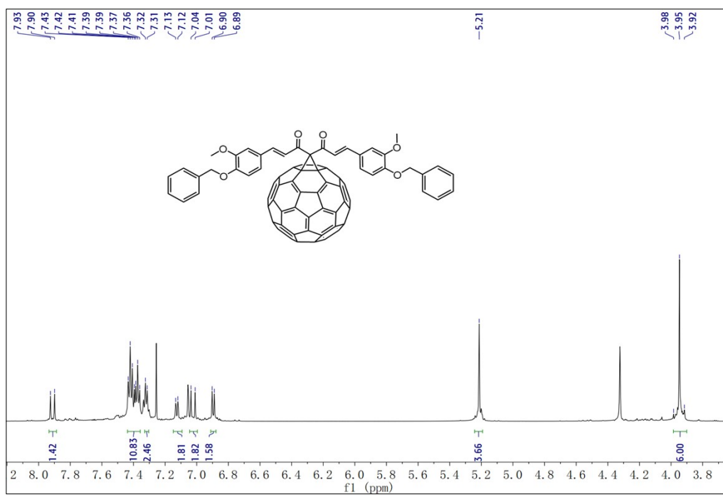
Fig. S10 ^1H NMR spectra of compound 2d
