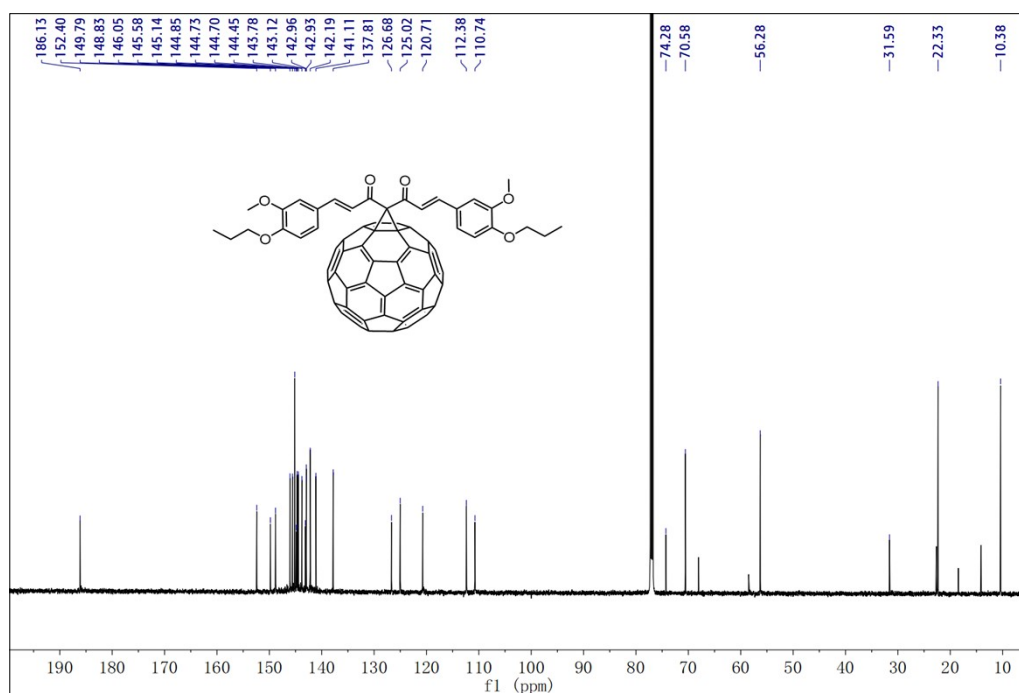
Fig. S5 13 C NMR spectra of compound 2b
