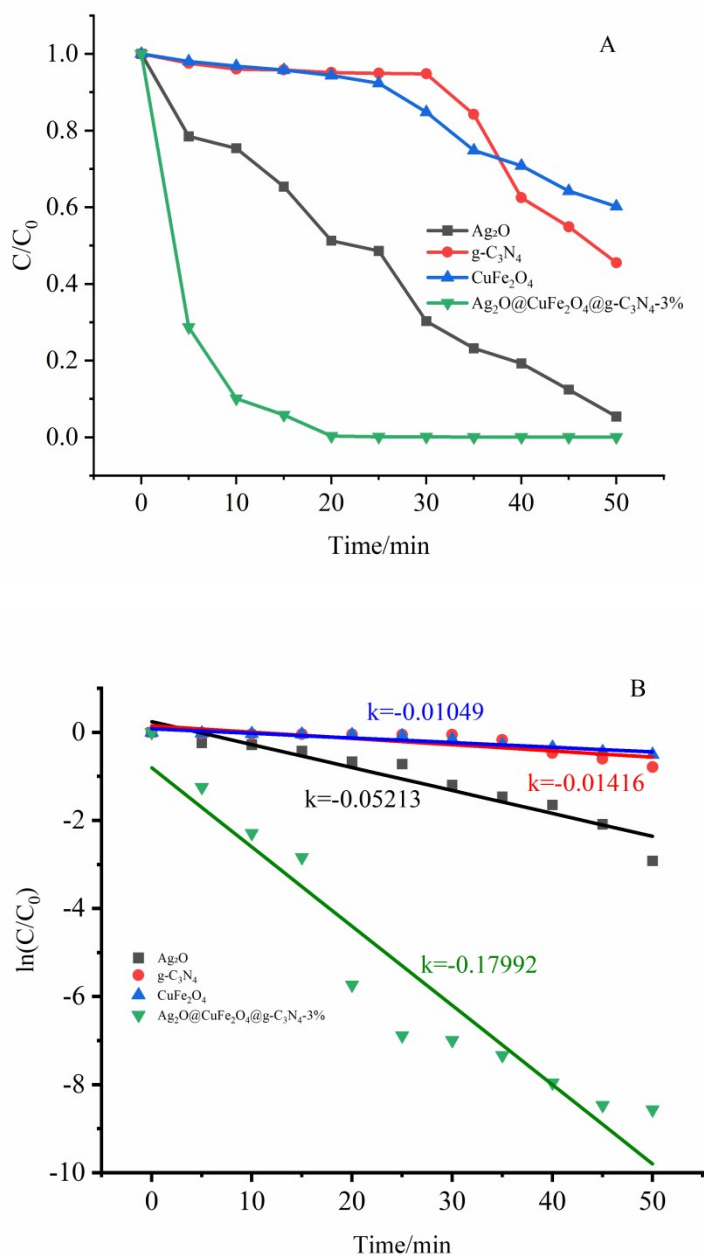
Fig. S1 The degradation curves of MB under visible lights change of (A) degradation rate, (B) kinetic plots with irradiated time.
