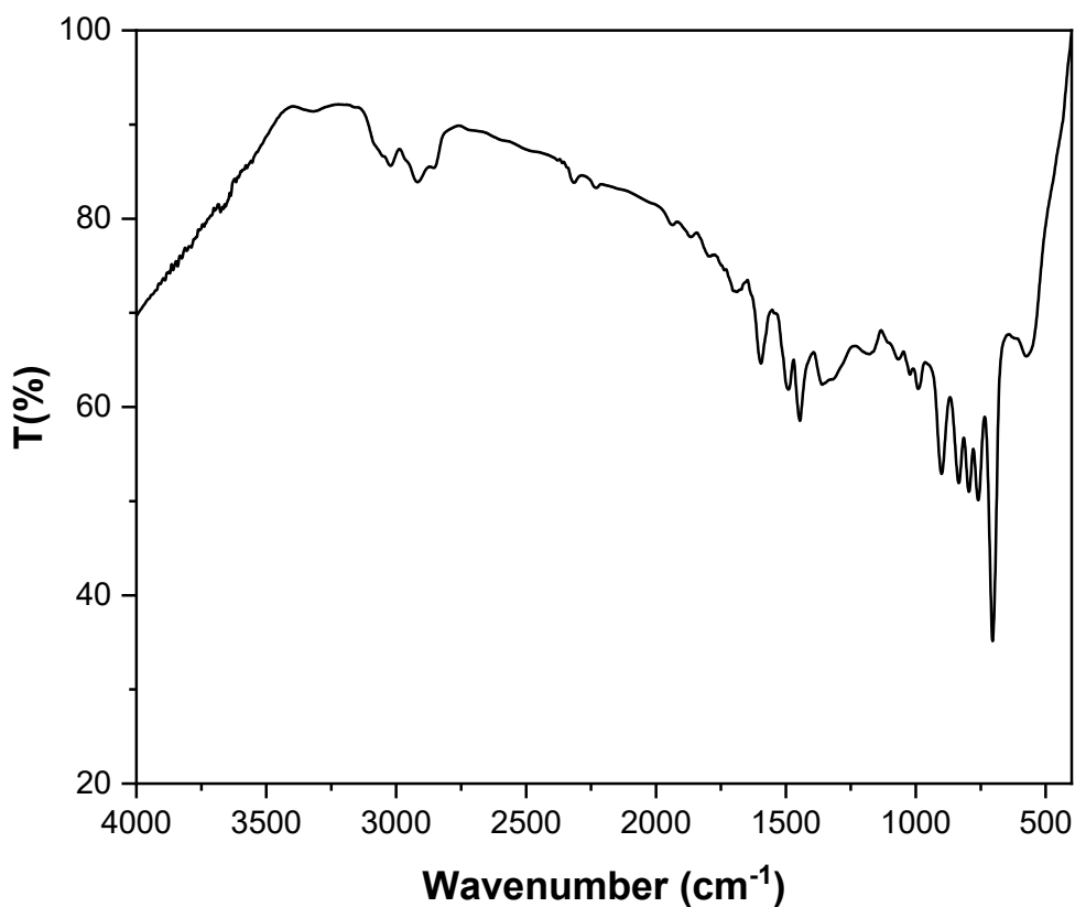
Figure S 1. FTIR spectra of poly(DVB) after adsorption of BG dye.
