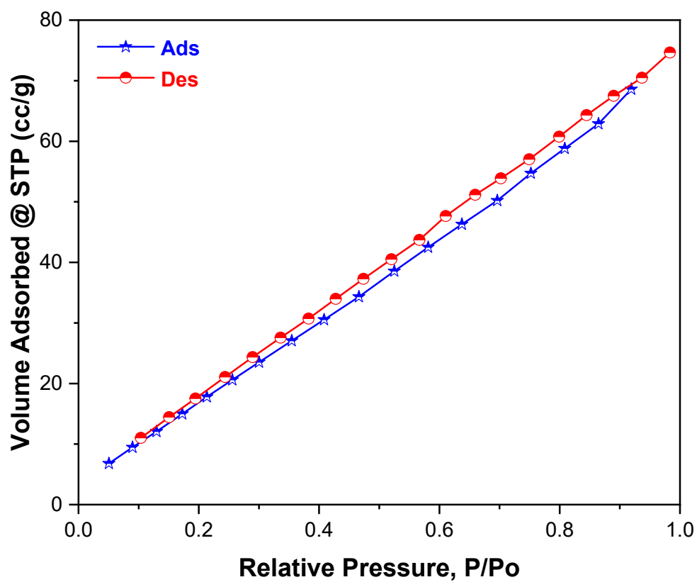
Figure S 2. BET analysis of poly(DVB) after adsorption of BG dye.
