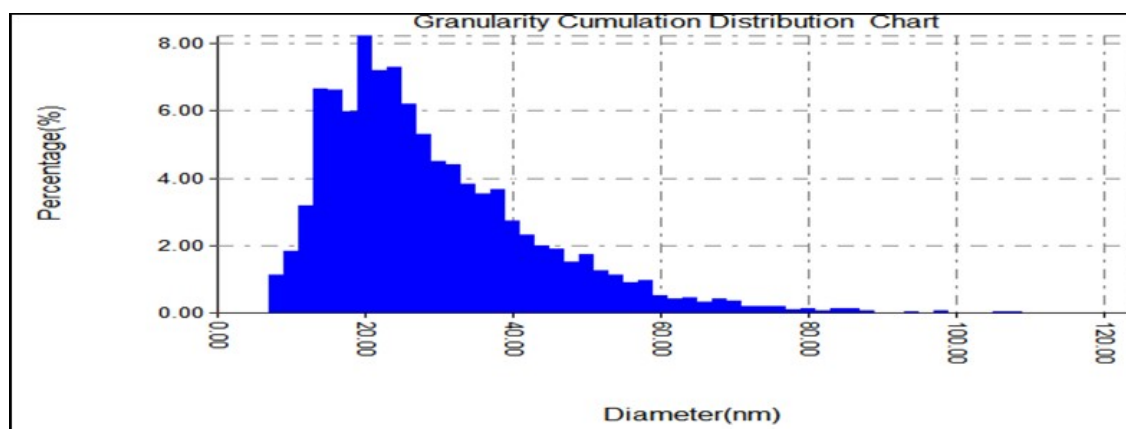
Figure S1: AFM Granularity Distribution Chart of ZnONPs.
