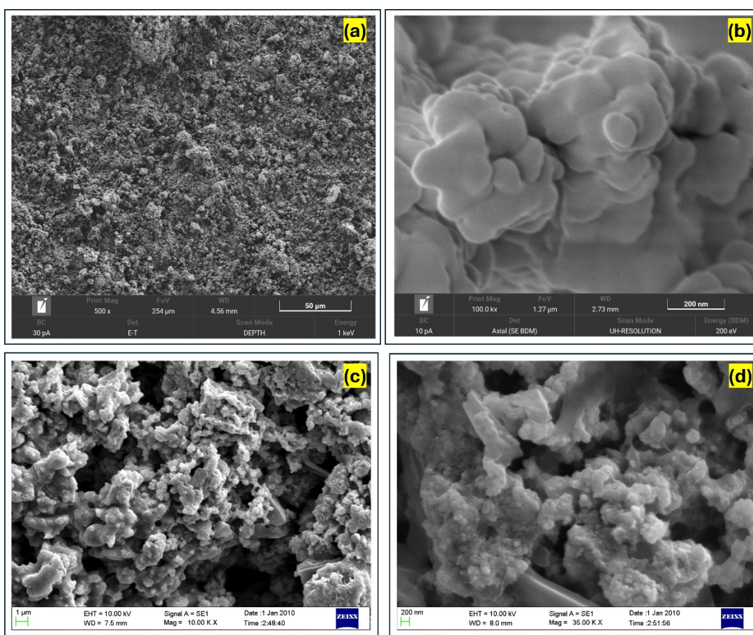
Figure. S2* FE-SEM images of (a) COP at lower resolution, (b) COP at higher resolution, (c) Mn 2 O 3 @COP at lower resolution, (d) Mn 2 O 3 @COP at higher resolution
