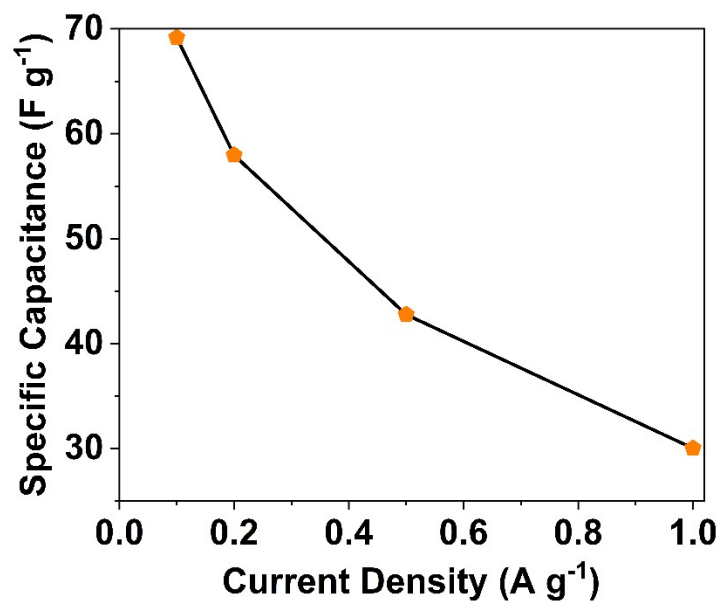
Figure. S3* Variation of specific capacitance with respect to current density of \text{Mn}_2\text{O}_3@\text{COP} electrode in 3 electrode system with 1M \text{H}_2\text{SO}_4 electrolyte
