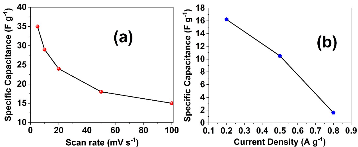
Figure. S4* (a) specific capacitance at various scan rates, (b) specific capacitance at various current densities.
