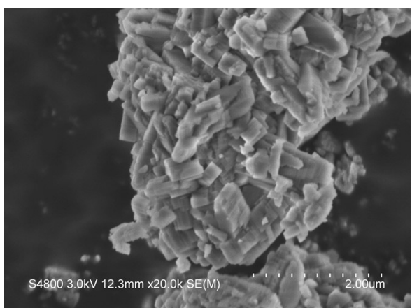
Figure S2 SEM images of commercial ZSM-5
